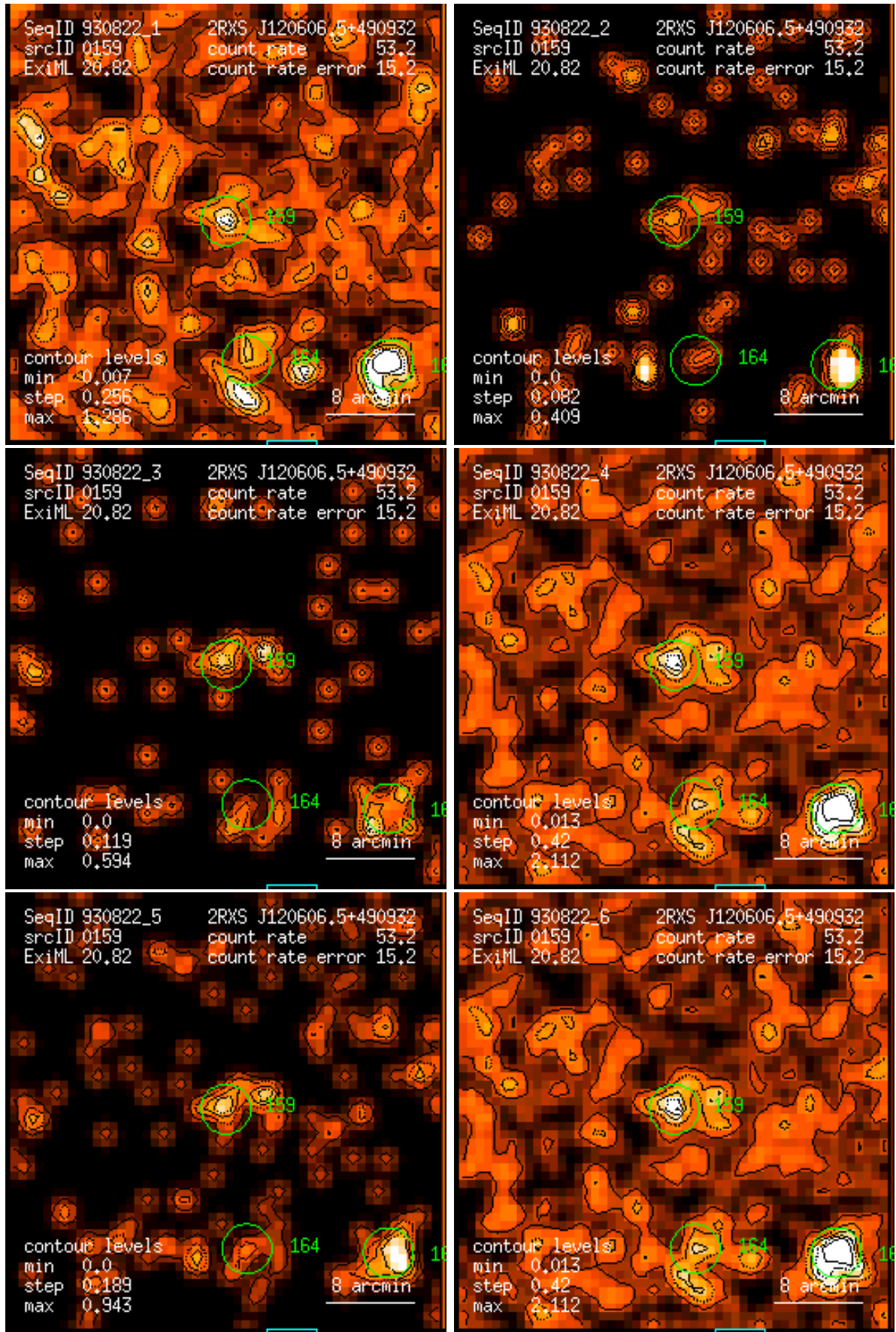
Figure 159: RASS 930822: detection 0159: band rate images, Gaussian filter: (1) PSPC channels 11 – 41, (2) 52 – 90, (3) 91 – 201, (4) 11 – 235, (5) 52 – 201, (6) 11 – 201. Broad band rates in counts/ks. Band rate contour levels in counts/ks/arcmin 2 .
