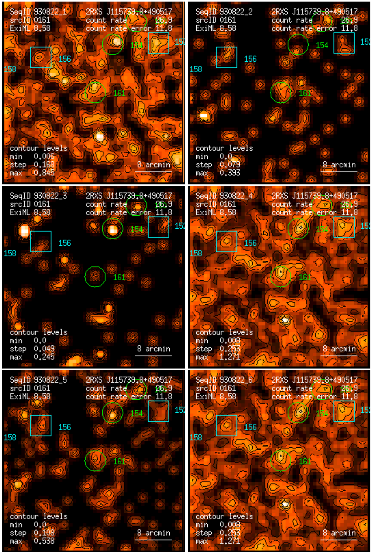
Figure 161: RASS 930822: detection 0161: band rate images, Gaussian filter: (1) PSPC channels 11 – 41, (2) 52 – 90, (3) 91 – 201, (4) 11 – 235, (5) 52 – 201, (6) 11 – 201. Broad band rates in counts/ks. Band rate contour levels in counts/ks/arcmin 2 .
