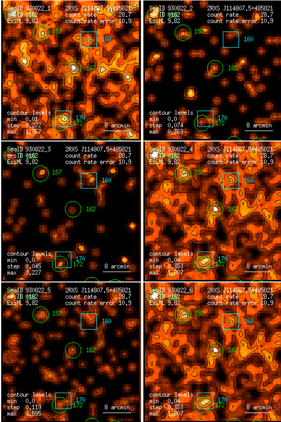
Figure 162: RASS 930822: detection 0162: band rate images, Gaussian filter: (1) PSPC channels 11 – 41, (2) 52 – 90, (3) 91 – 201, (4) 11 – 235, (5) 52 – 201, (6) 11 – 201. Broad band rates in counts/ks. Band rate contour levels in counts/ks/arcmin 2 .
