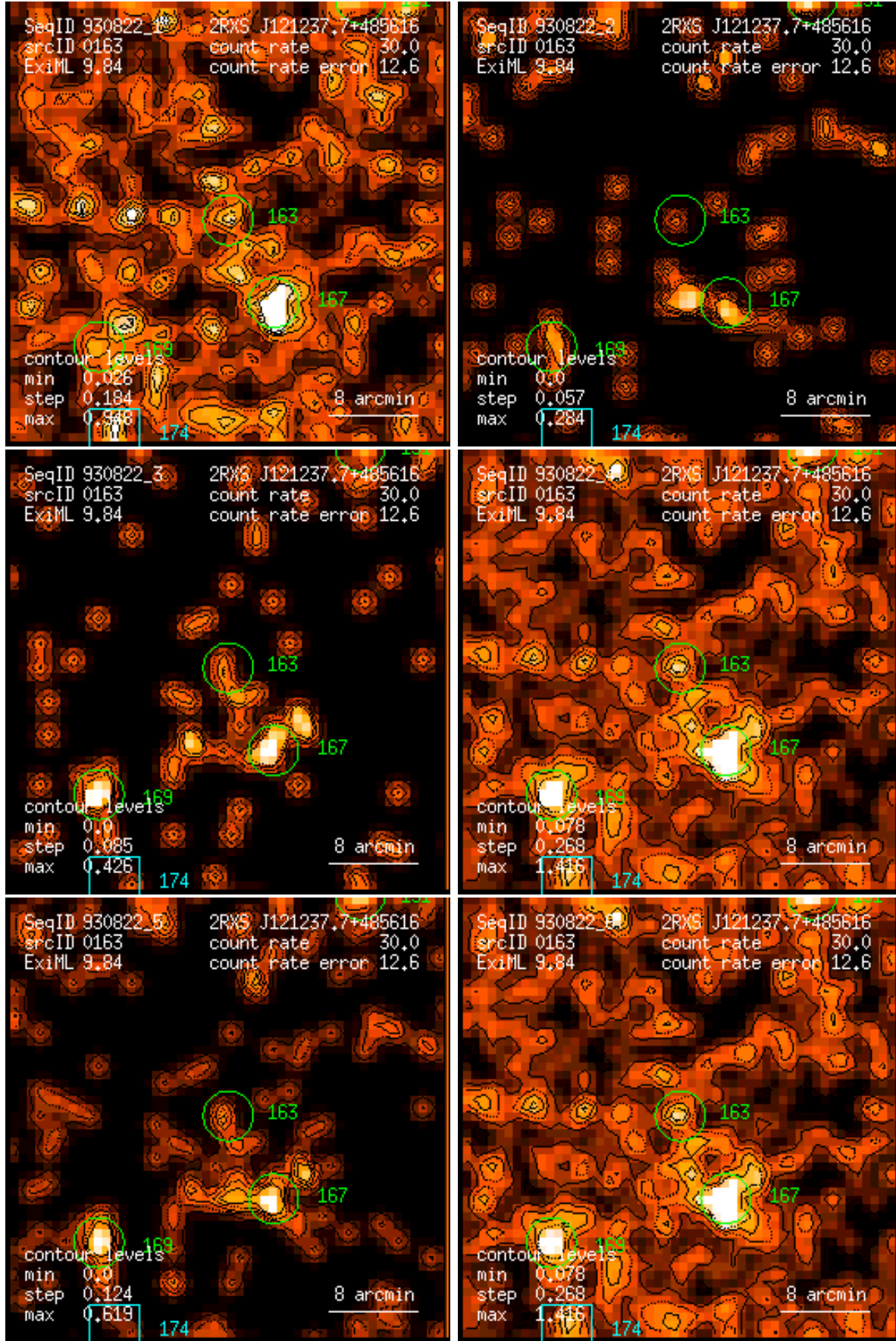
Figure 163: RASS 930822: detection 0163: band rate images, Gaussian filter: (1) PSPC channels 11 – 41, (2) 52 – 90, (3) 91 – 201, (4) 11 – 235, (5) 52 – 201, (6) 11 – 201. Broad band rates in counts/ks. Band rate contour levels in counts/ks/arcmin 2 .
