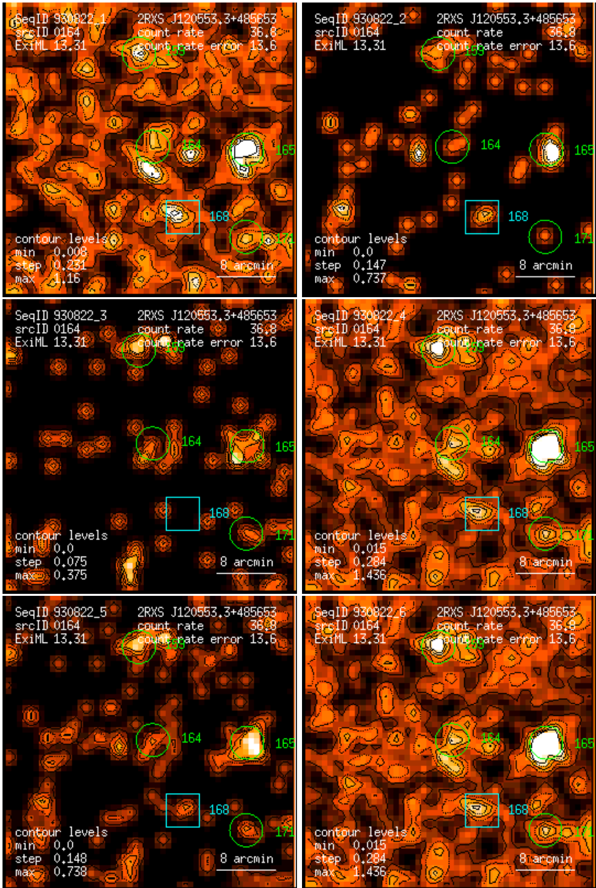
Figure 164: RASS 930822: detection 0164: band rate images, Gaussian filter: (1) PSPC channels 11 – 41, (2) 52 – 90, (3) 91 – 201, (4) 11 – 235, (5) 52 – 201, (6) 11 – 201. Broad band rates in counts/ks. Band rate contour levels in counts/ks/arcmin 2 .
