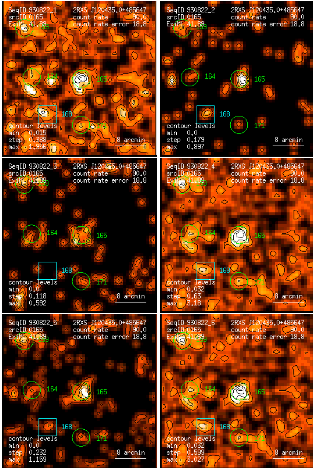
Figure 165: RASS 930822: detection 0165: band rate images, Gaussian filter: (1) PSPC channels 11 – 41, (2) 52 – 90, (3) 91 – 201, (4) 11 – 235, (5) 52 – 201, (6) 11 – 201. Broad band rates in counts/ks. Band rate contour levels in counts/ks/arcmin 2 .
