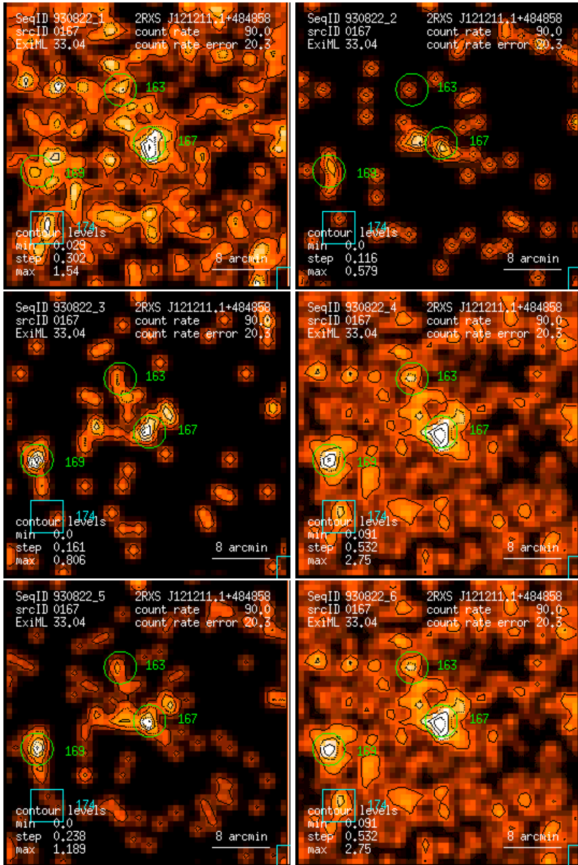
Figure 167: RASS 930822: detection 0167: band rate images, Gaussian filter: (1) PSPC channels 11 – 41, (2) 52 – 90, (3) 91 – 201, (4) 11 – 235, (5) 52 – 201, (6) 11 – 201. Broad band rates in counts/ks. Band rate contour levels in counts/ks/arcmin 2 .
