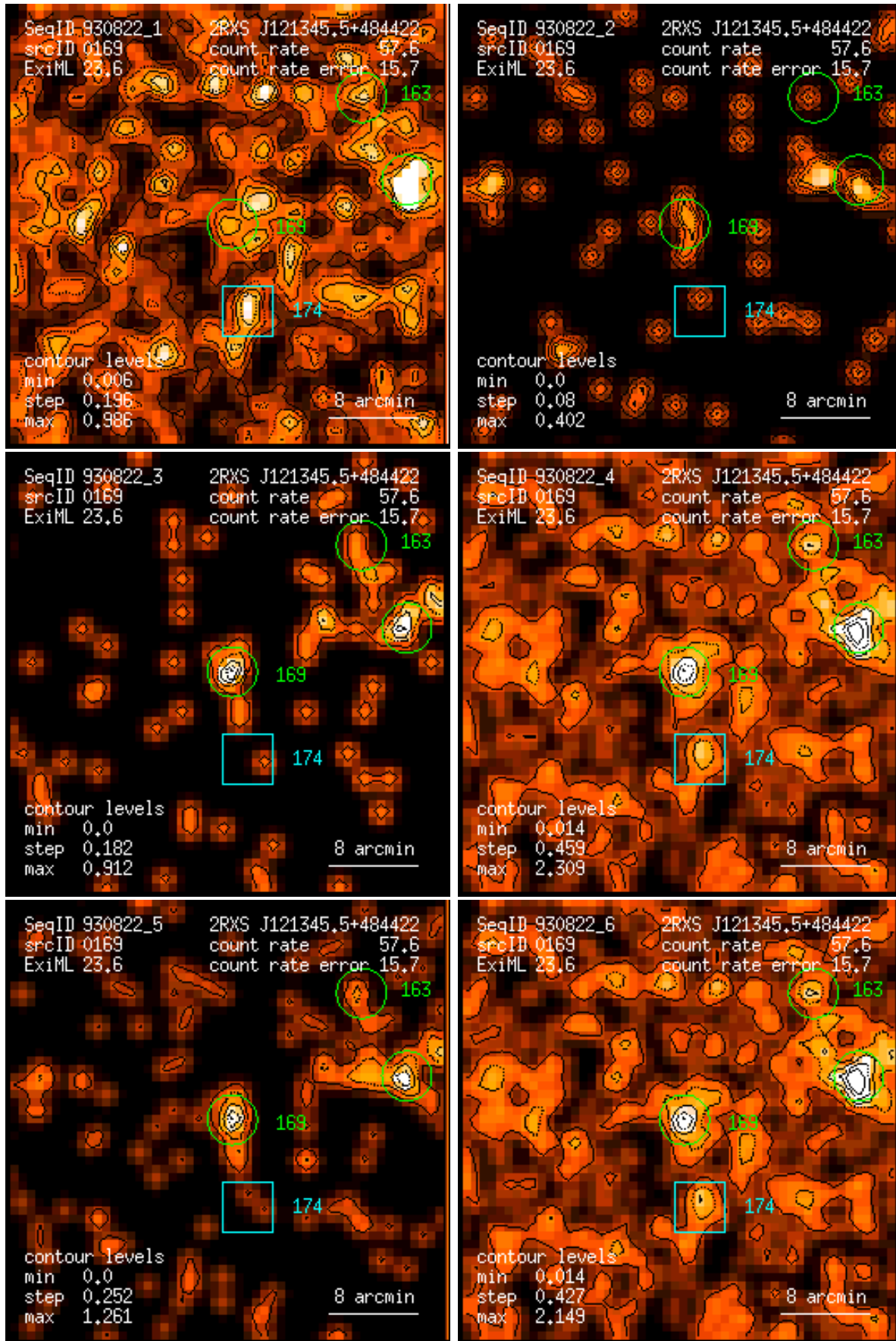
Figure 169: RASS 930822: detection 0169: band rate images, Gaussian filter: (1) PSPC channels 11 – 41, (2) 52 – 90, (3) 91 – 201, (4) 11 – 235, (5) 52 – 201, (6) 11 – 201. Broad band rates in counts/ks. Band rate contour levels in counts/ks/arcmin 2 .
