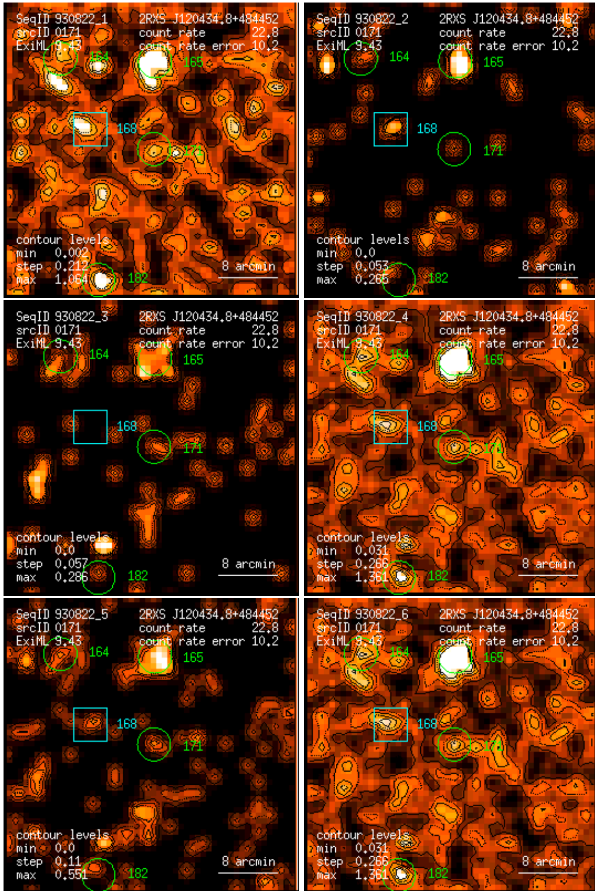
Figure 171: RASS 930822: detection 0171: band rate images, Gaussian filter: (1) PSPC channels 11 – 41, (2) 52 – 90, (3) 91 – 201, (4) 11 – 235, (5) 52 – 201, (6) 11 – 201. Broad band rates in counts/ks. Band rate contour levels in counts/ks/arcmin 2 .
