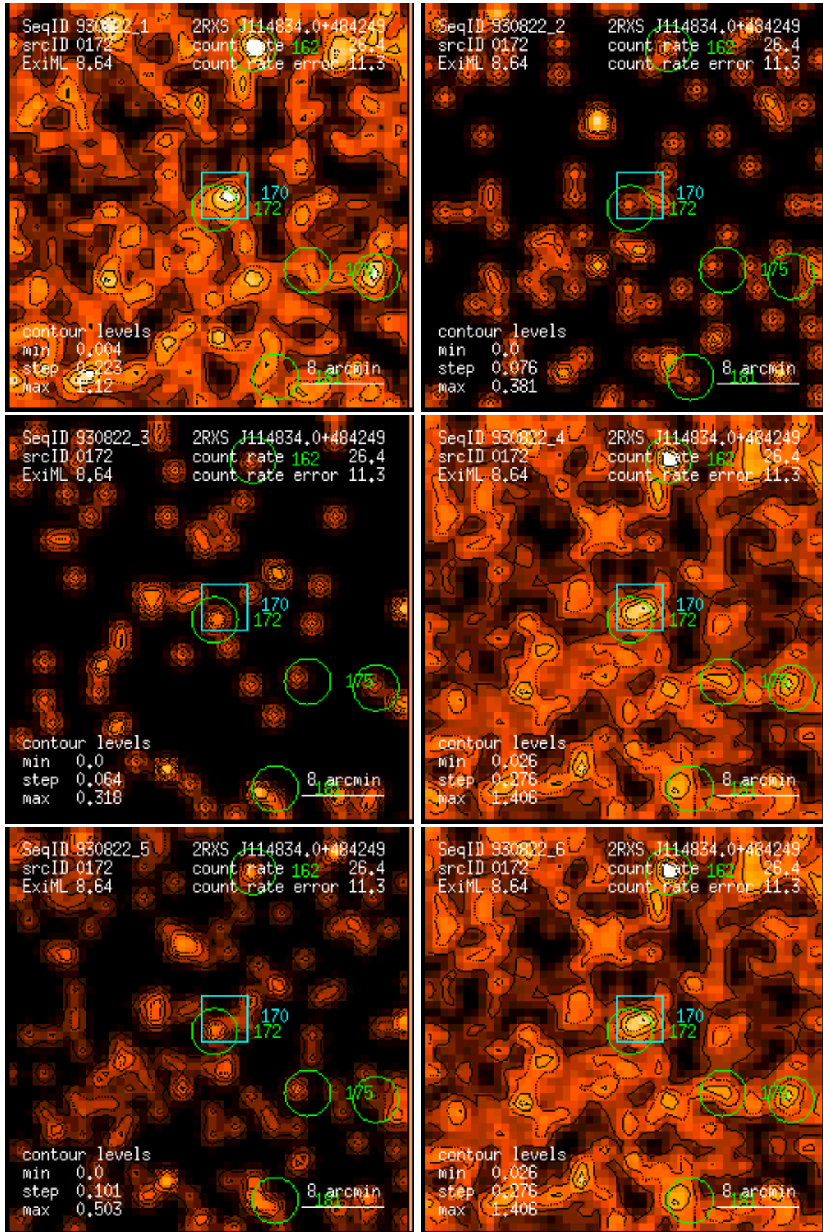
Figure 172: RASS 930822: detection 0172: band rate images, Gaussian filter: (1) PSPC channels 11 – 41, (2) 52 – 90, (3) 91 – 201, (4) 11 – 235, (5) 52 – 201, (6) 11 – 201. Broad band rates in counts/ks. Band rate contour levels in counts/ks/arcmin 2 .
