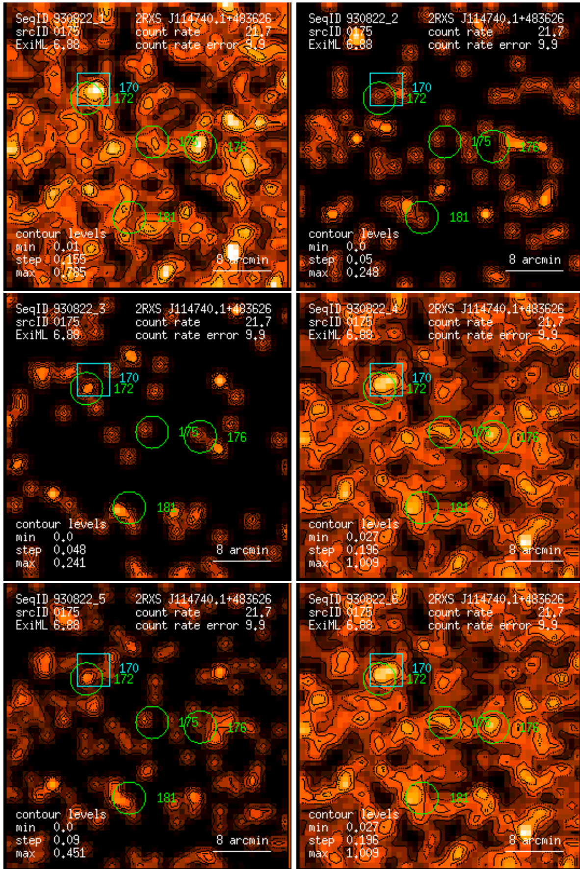
Figure 175: RASS 930822: detection 0175: band rate images, Gaussian filter: (1) PSPC channels 11 – 41, (2) 52 – 90, (3) 91 – 201, (4) 11 – 235, (5) 52 – 201, (6) 11 – 201. Broad band rates in counts/ks. Band rate contour levels in counts/ks/arcmin 2 .
