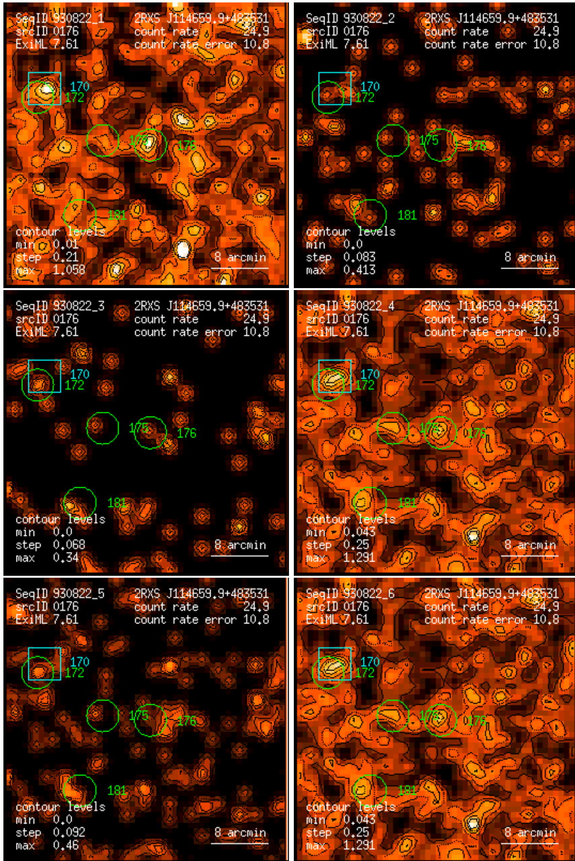
Figure 176: RASS 930822: detection 0176: band rate images, Gaussian filter: (1) PSPC channels 11 – 41, (2) 52 – 90, (3) 91 – 201, (4) 11 – 235, (5) 52 – 201, (6) 11 – 201. Broad band rates in counts/ks. Band rate contour levels in counts/ks/arcmin 2 .
