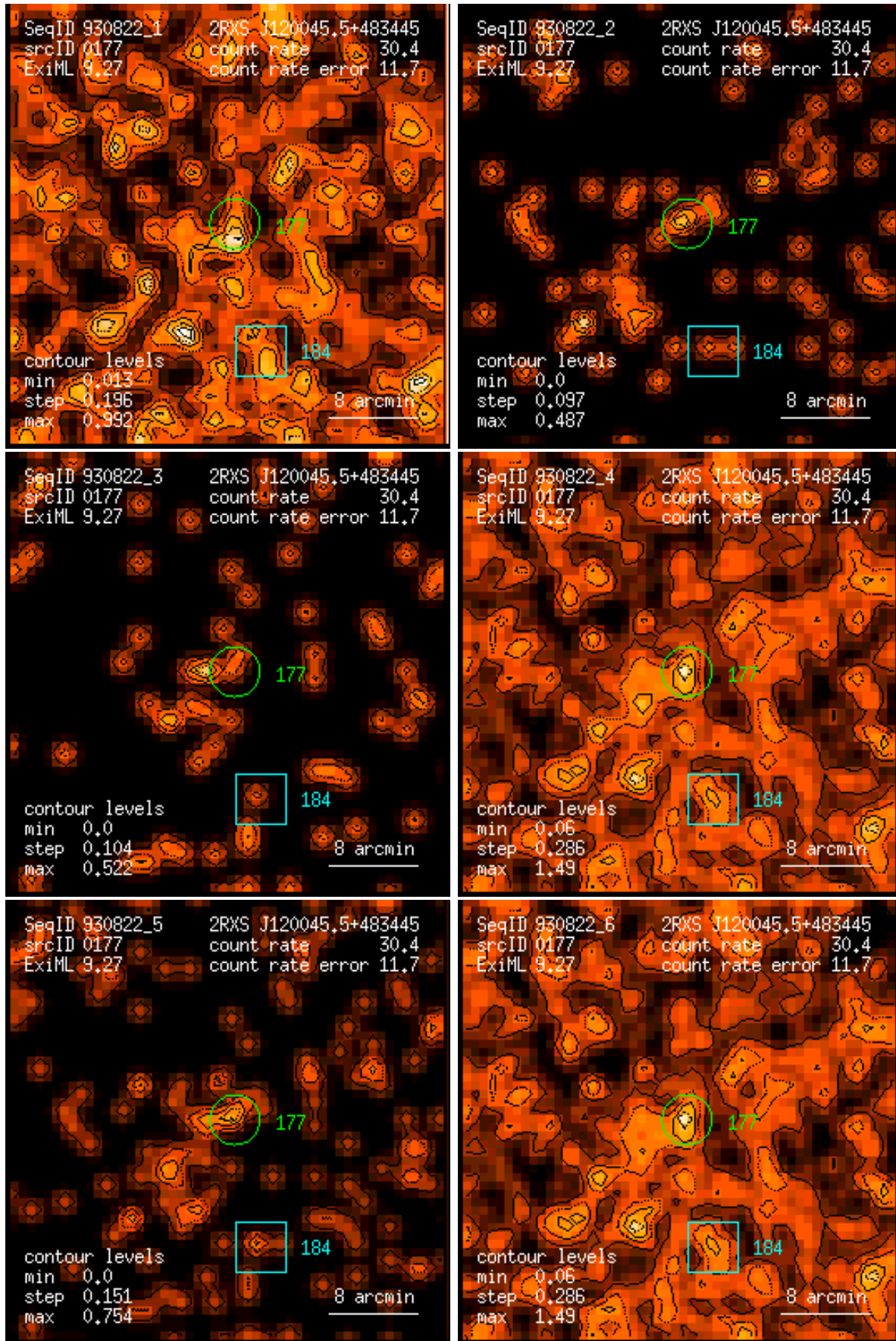
Figure 177: RASS 930822: detection 0177: band rate images, Gaussian filter: (1) PSPC channels 11 – 41, (2) 52 – 90, (3) 91 – 201, (4) 11 – 235, (5) 52 – 201, (6) 11 – 201. Broad band rates in counts/ks. Band rate contour levels in counts/ks/arcmin 2 .
