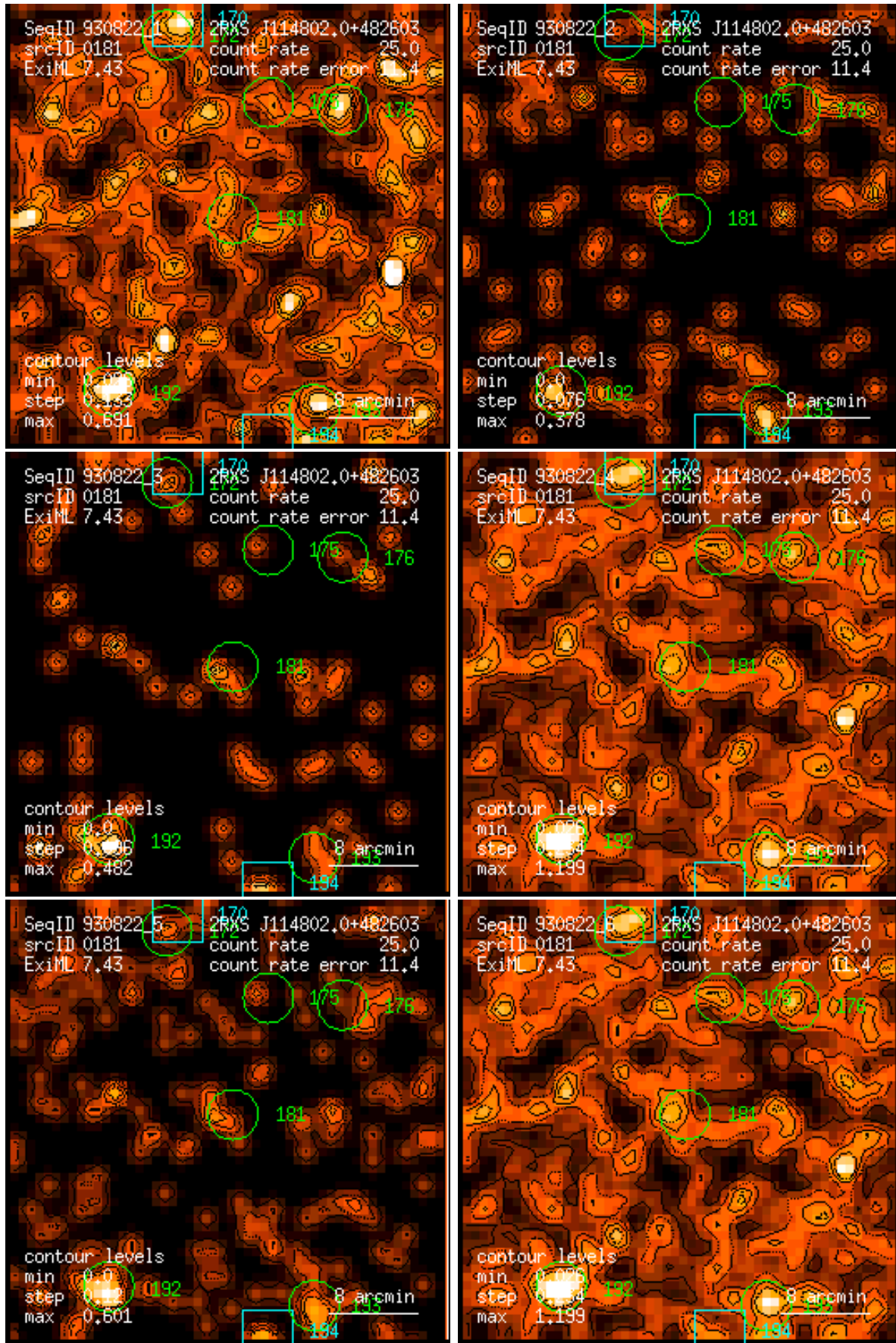
Figure 181: RASS 930822: detection 0181: band rate images, Gaussian filter: (1) PSPC channels 11 – 41, (2) 52 – 90, (3) 91 – 201, (4) 11 – 235, (5) 52 – 201, (6) 11 – 201. Broad band rates in counts/ks. Band rate contour levels in counts/ks/arcmin 2 .
