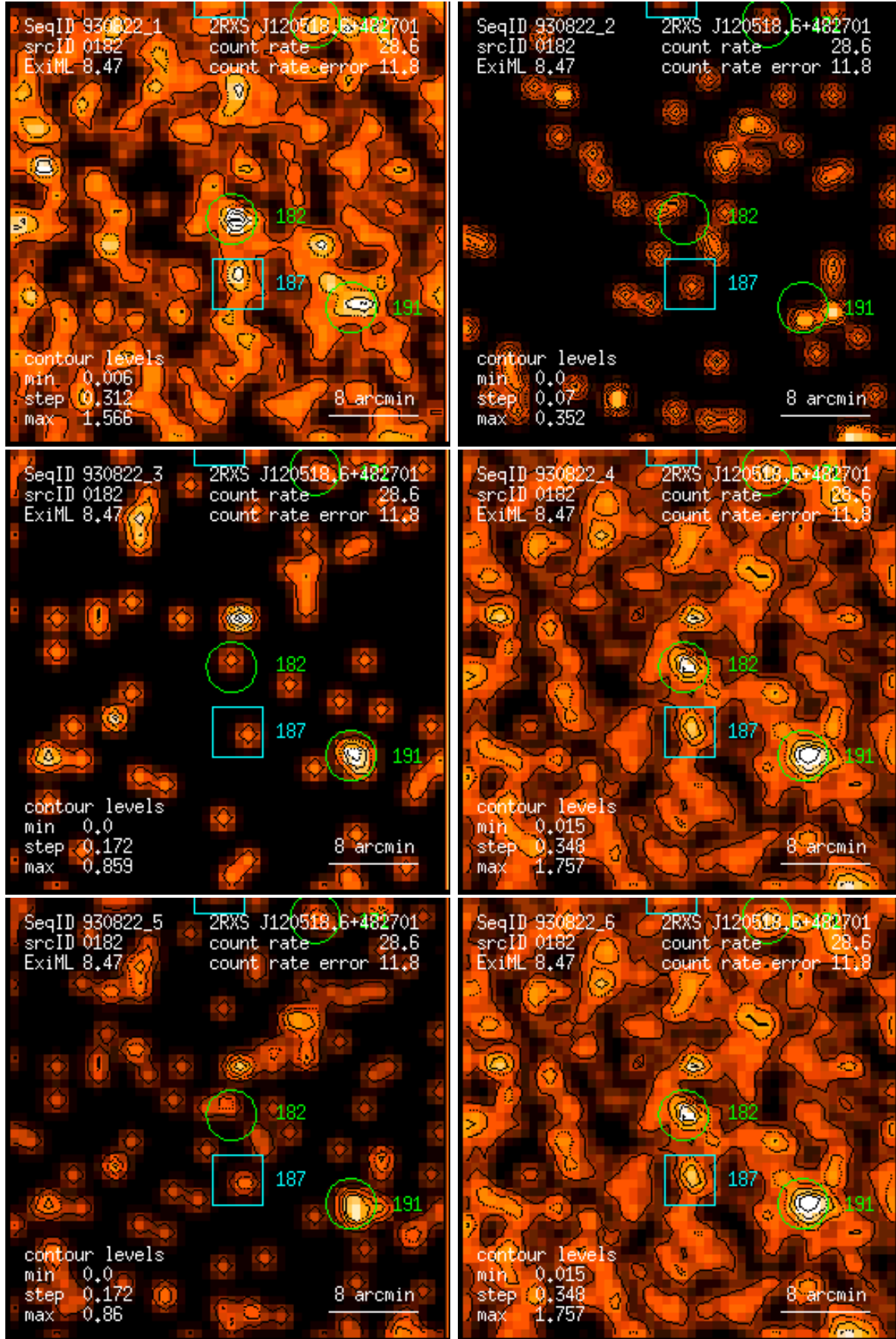
Figure 182: RASS 930822: detection 0182: band rate images, Gaussian filter: (1) PSPC channels 11 – 41, (2) 52 – 90, (3) 91 – 201, (4) 11 – 235, (5) 52 – 201, (6) 11 – 201. Broad band rates in counts/ks. Band rate contour levels in counts/ks/arcmin 2 .
