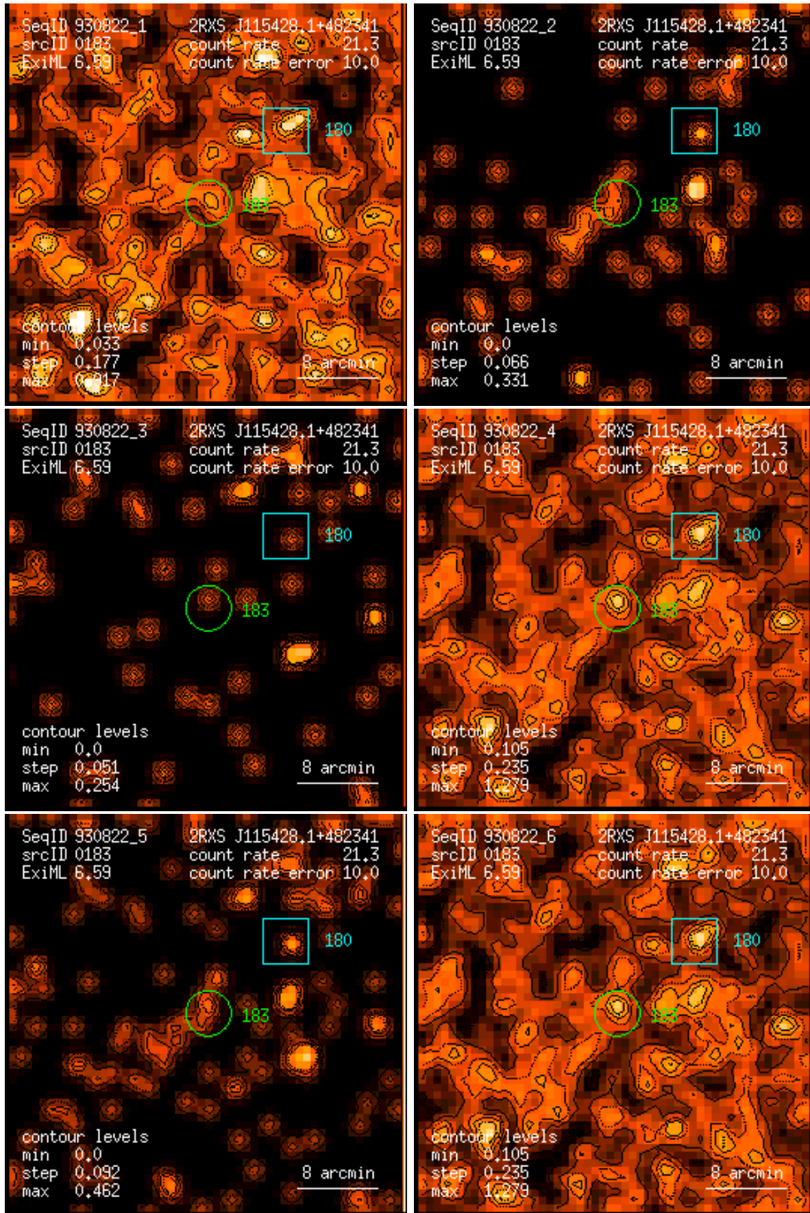
Figure 183: RASS 930822: detection 0183: band rate images, Gaussian filter: (1) PSPC channels 11 – 41, (2) 52 – 90, (3) 91 – 201, (4) 11 – 235, (5) 52 – 201, (6) 11 – 201. Broad band rates in counts/ks. Band rate contour levels in counts/ks/arcmin 2 .
