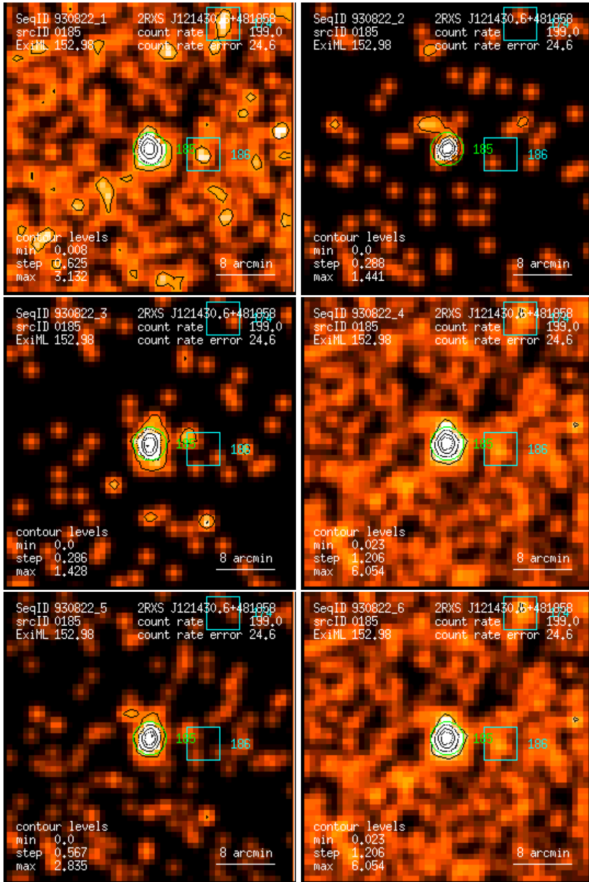
Figure 185: RASS 930822: detection 0185: band rate images, Gaussian filter: (1) PSPC channels 11 – 41, (2) 52 – 90, (3) 91 – 201, (4) 11 – 235, (5) 52 – 201, (6) 11 – 201. Broad band rates in counts/ks. Band rate contour levels in counts/ks/arcmin 2 .
