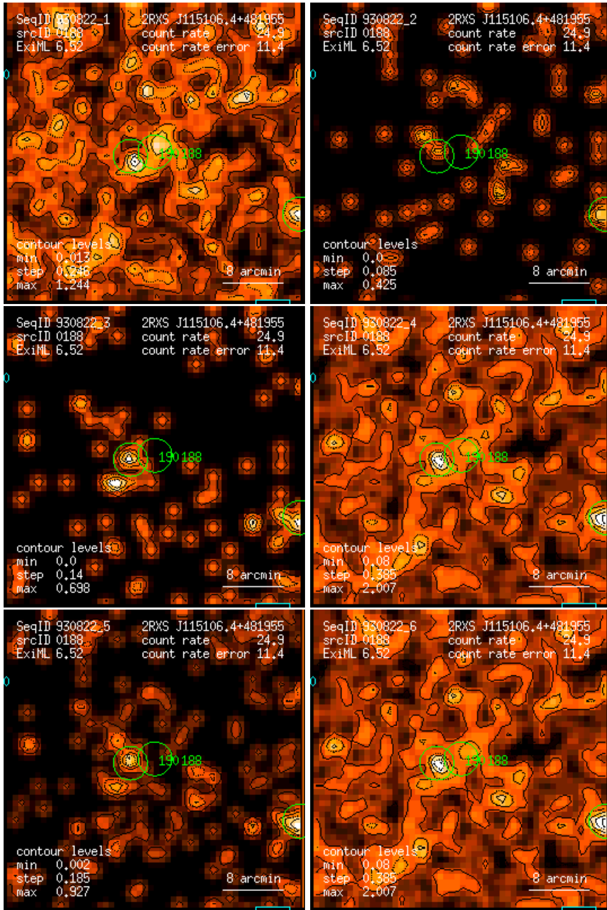
Figure 188: RASS 930822: detection 0188: band rate images, Gaussian filter: (1) PSPC channels 11 – 41, (2) 52 – 90, (3) 91 – 201, (4) 11 – 235, (5) 52 – 201, (6) 11 – 201. Broad band rates in counts/ks. Band rate contour levels in counts/ks/arcmin 2 .
