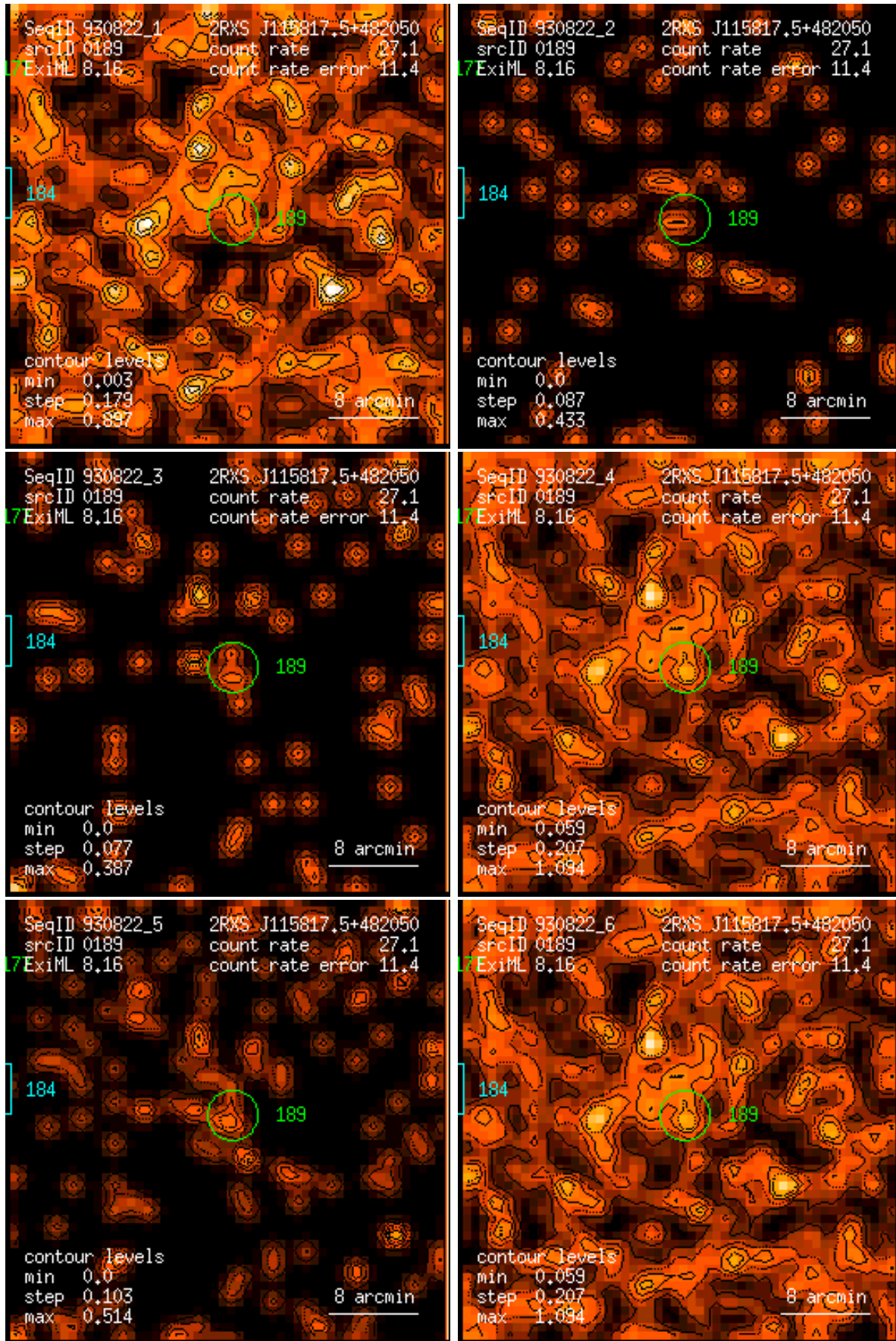
Figure 189: RASS 930822: detection 0189: band rate images, Gaussian filter: (1) PSPC channels 11 – 41, (2) 52 – 90, (3) 91 – 201, (4) 11 – 235, (5) 52 – 201, (6) 11 – 201. Broad band rates in counts/ks. Band rate contour levels in counts/ks/arcmin 2 .
