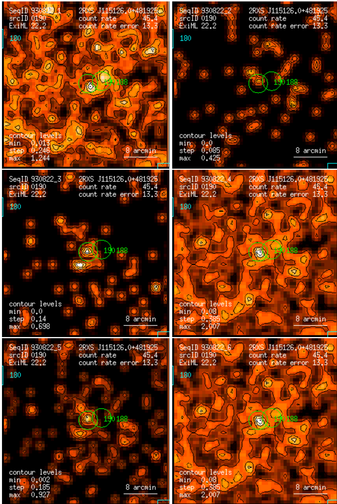
Figure 190: RASS 930822: detection 0190: band rate images, Gaussian filter: (1) PSPC channels 11 – 41, (2) 52 – 90, (3) 91 – 201, (4) 11 – 235, (5) 52 – 201, (6) 11 – 201. Broad band rates in counts/ks. Band rate contour levels in counts/ks/arcmin 2 .
