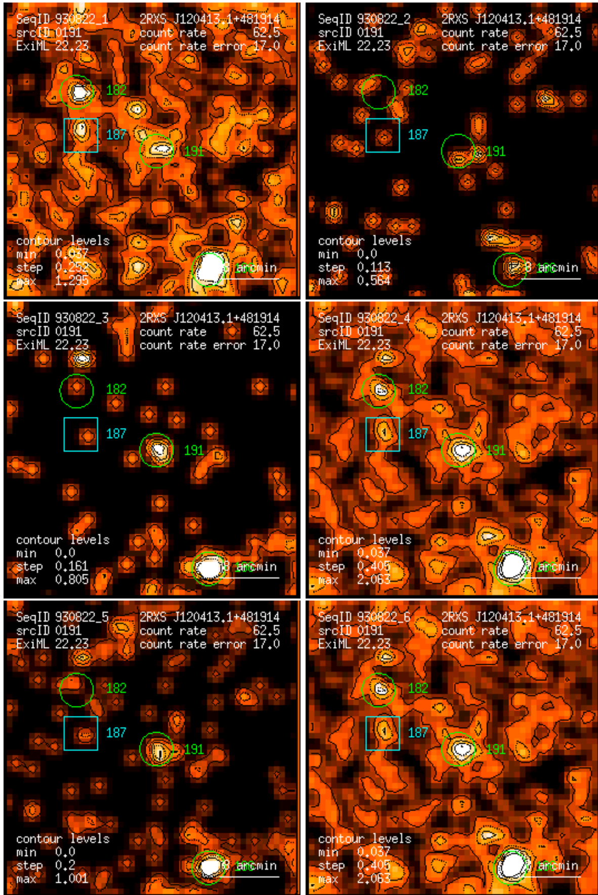
Figure 191: RASS 930822: detection 0191: band rate images, Gaussian filter: (1) PSPC channels 11 – 41, (2) 52 – 90, (3) 91 – 201, (4) 11 – 235, (5) 52 – 201, (6) 11 – 201. Broad band rates in counts/ks. Band rate contour levels in counts/ks/arcmin 2 .
