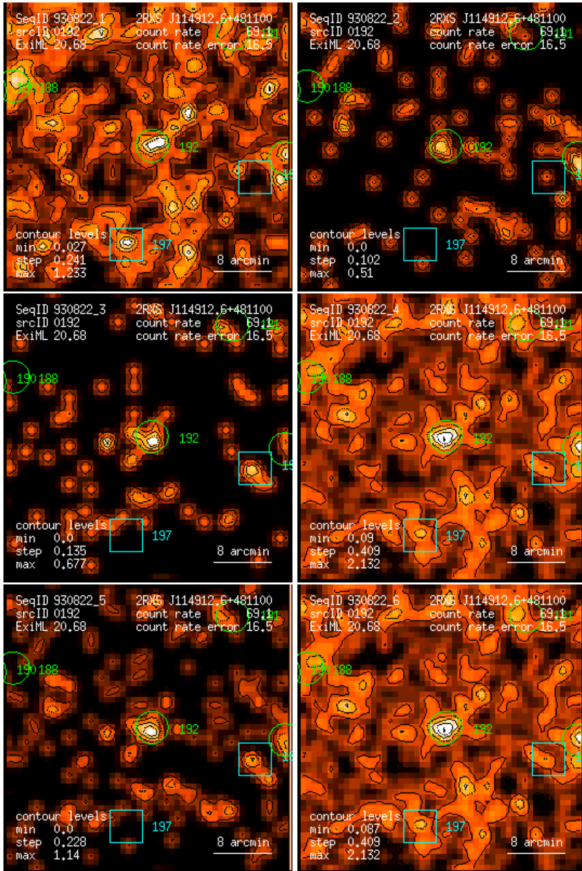
Figure 192: RASS 930822: detection 0192: band rate images, Gaussian filter: (1) PSPC channels 11 – 41, (2) 52 – 90, (3) 91 – 201, (4) 11 – 235, (5) 52 – 201, (6) 11 – 201. Broad band rates in counts/ks. Band rate contour levels in counts/ks/arcmin 2 .
