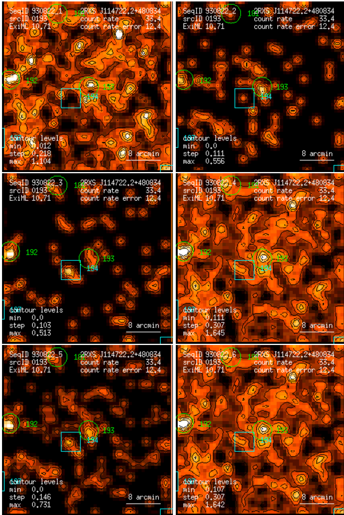
Figure 193: RASS 930822: detection 0193: band rate images, Gaussian filter: (1) PSPC channels 11 – 41, (2) 52 – 90, (3) 91 – 201, (4) 11 – 235, (5) 52 – 201, (6) 11 – 201. Broad band rates in counts/ks. Band rate contour levels in counts/ks/arcmin 2 .
