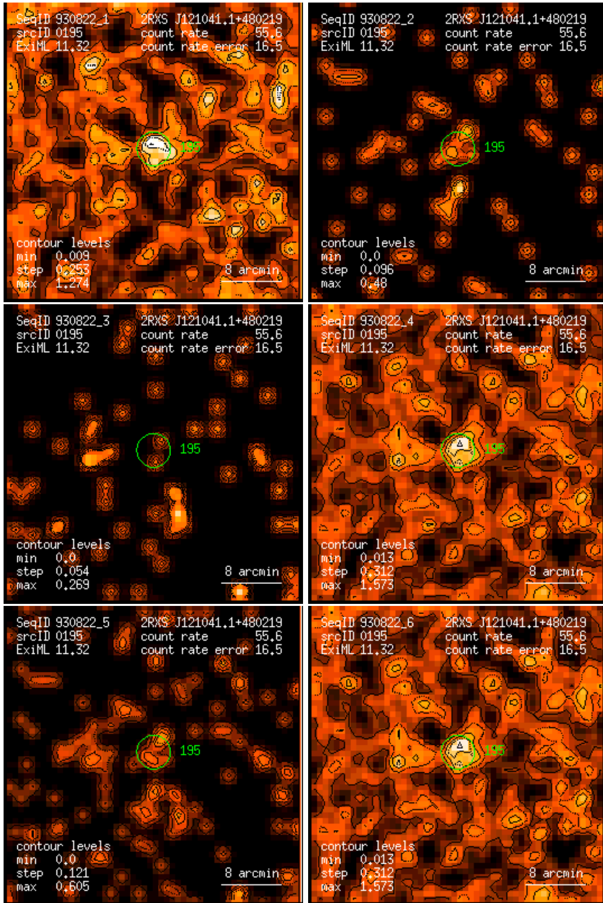
Figure 195: RASS 930822: detection 0195: band rate images, Gaussian filter: (1) PSPC channels 11 – 41, (2) 52 – 90, (3) 91 – 201, (4) 11 – 235, (5) 52 – 201, (6) 11 – 201. Broad band rates in counts/ks. Band rate contour levels in counts/ks/arcmin 2 .
