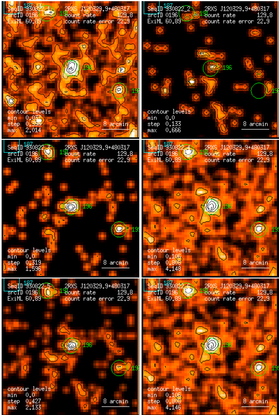
Figure 196: RASS 930822: detection 0196: band rate images, Gaussian filter: (1) PSPC channels 11 – 41, (2) 52 – 90, (3) 91 – 201, (4) 11 – 235, (5) 52 – 201, (6) 11 – 201. Broad band rates in counts/ks. Band rate contour levels in counts/ks/arcmin 2 .
