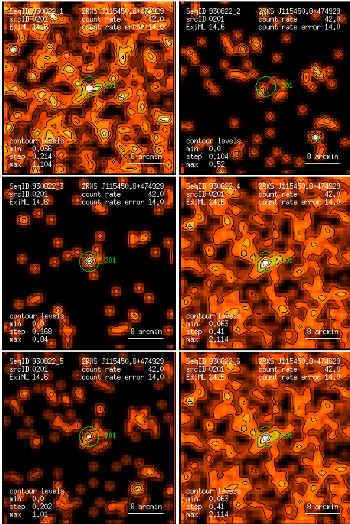
Figure 201: RASS 930822: detection 0201: band rate images, Gaussian filter: (1) PSPC channels 11 – 41, (2) 52 – 90, (3) 91 – 201, (4) 11 – 235, (5) 52 – 201, (6) 11 – 201. Broad band rates in counts/ks. Band rate contour levels in counts/ks/arcmin 2 .
