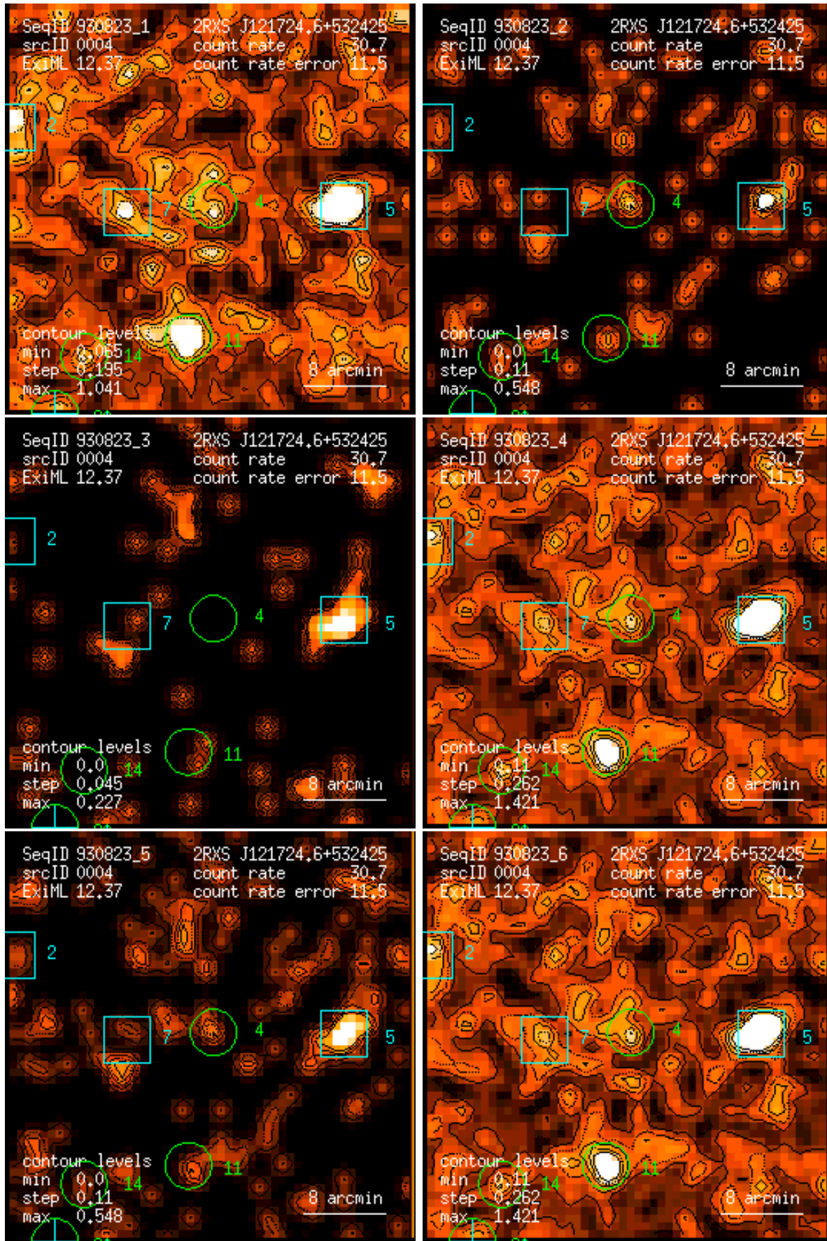
Figure 4: RASS 930823: detection 0004: band rate images, Gaussian filter: (1) PSPC channels 11 – 41, (2) 52 – 90, (3) 91 – 201, (4) 11 – 235, (5) 52 – 201, (6) 11 – 201. Broad band rates in counts/ks. Band rate contour levels in counts/ks/arcmin 2 .
