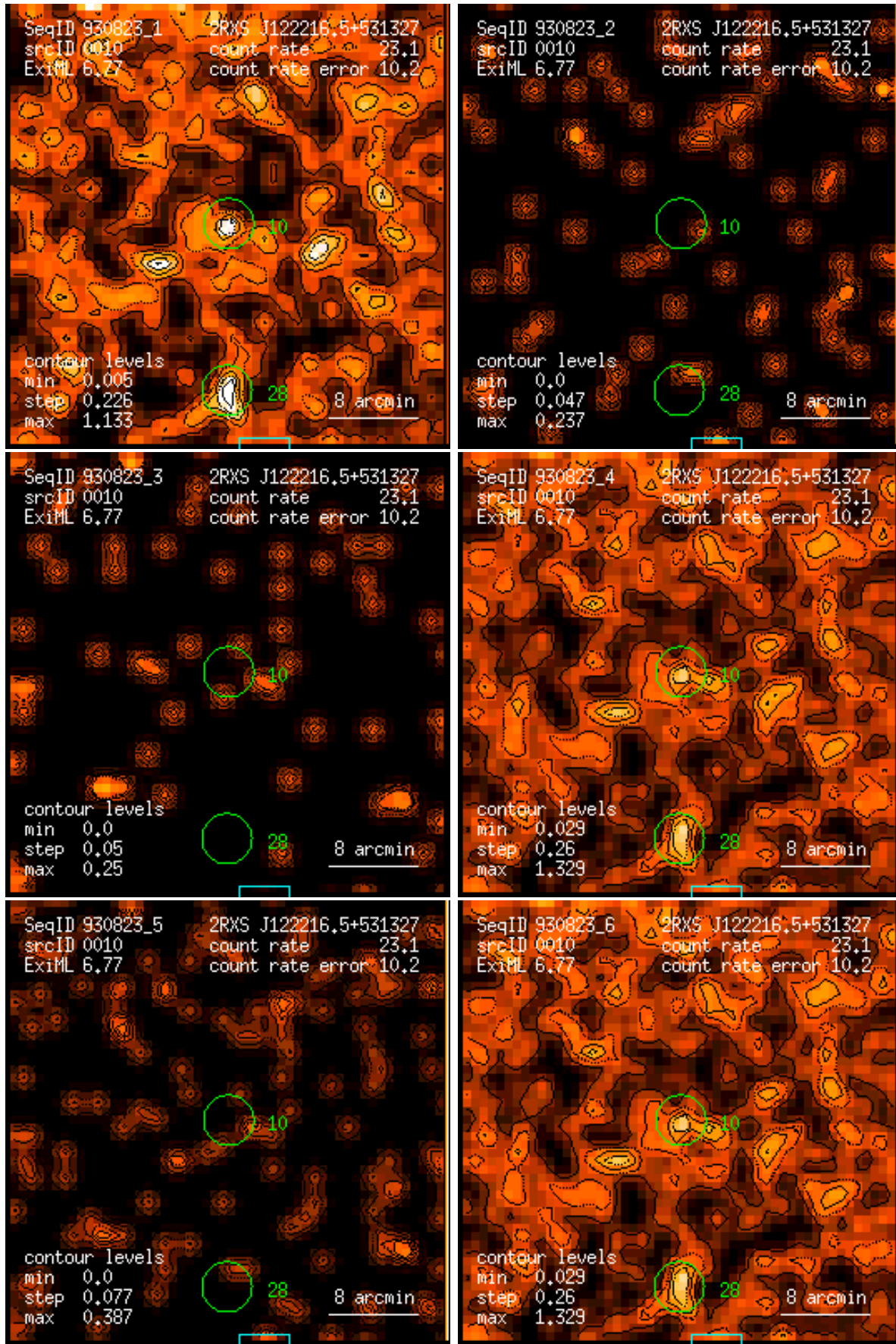
Figure 10: RASS 930823: detection 0010: band rate images, Gaussian filter: (1) PSPC channels 11 – 41, (2) 52 – 90, (3) 91 – 201, (4) 11 – 235, (5) 52 – 201, (6) 11 – 201. Broad band rates in counts/ks. Band rate contour levels in counts/ks/arcmin 2 .
