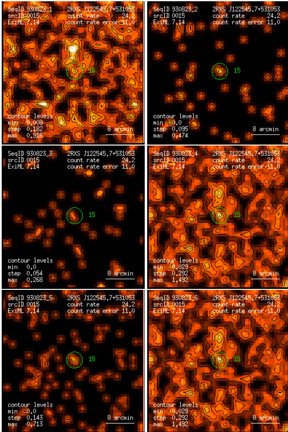
Figure 15: RASS 930823: detection 0015: band rate images, Gaussian filter: (1) PSPC channels 11 – 41, (2) 52 – 90, (3) 91 – 201, (4) 11 – 235, (5) 52 – 201, (6) 11 – 201. Broad band rates in counts/ks. Band rate contour levels in counts/ks/arcmin 2 .
