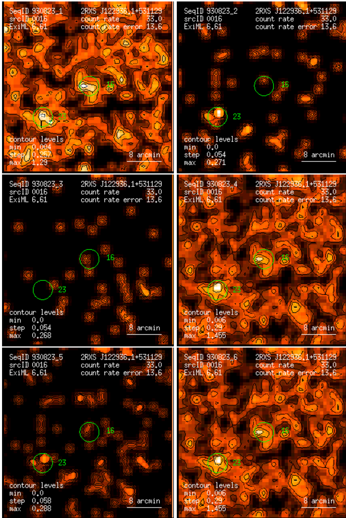
Figure 16: RASS 930823: detection 0016: band rate images, Gaussian filter: (1) PSPC channels 11 – 41, (2) 52 – 90, (3) 91 – 201, (4) 11 – 235, (5) 52 – 201, (6) 11 – 201. Broad band rates in counts/ks. Band rate contour levels in counts/ks/arcmin 2 .
