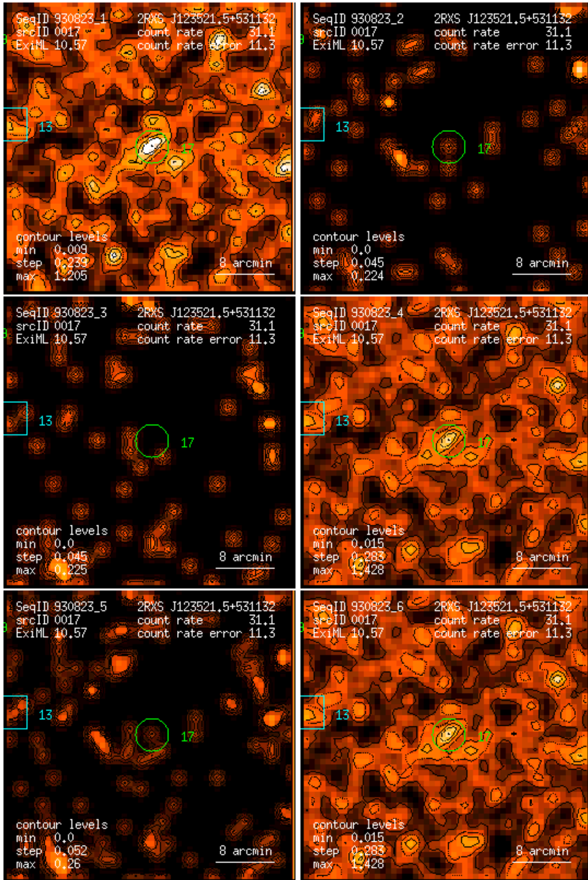
Figure 17: RASS 930823: detection 0017: band rate images, Gaussian filter: (1) PSPC channels 11 – 41, (2) 52 – 90, (3) 91 – 201, (4) 11 – 235, (5) 52 – 201, (6) 11 – 201. Broad band rates in counts/ks. Band rate contour levels in counts/ks/arcmin 2 .
