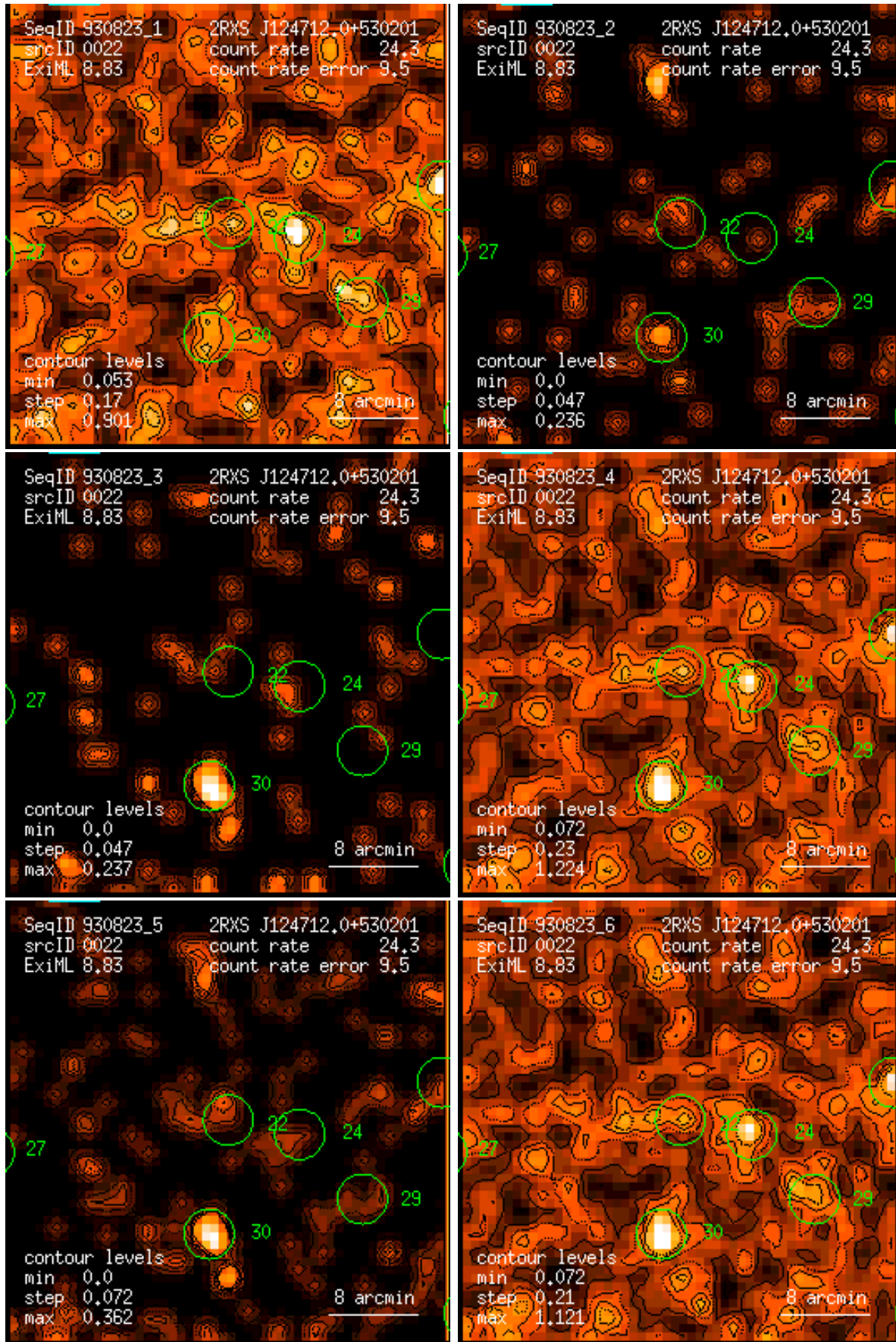
Figure 22: RASS 930823: detection 0022: band rate images, Gaussian filter: (1) PSPC channels 11 – 41, (2) 52 – 90, (3) 91 – 201, (4) 11 – 235, (5) 52 – 201, (6) 11 – 201. Broad band rates in counts/ks. Band rate contour levels in counts/ks/arcmin 2 .
