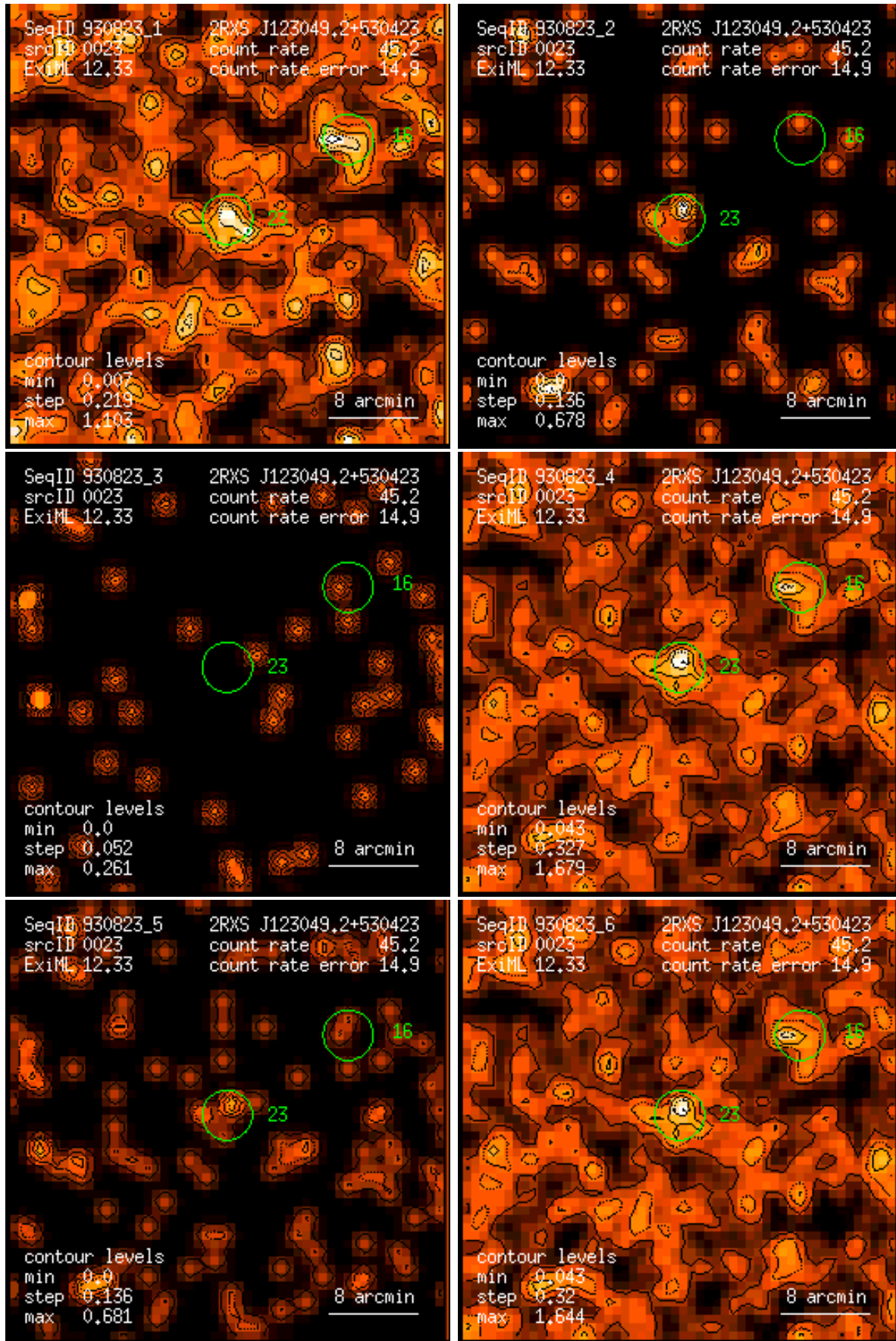
Figure 23: RASS 930823: detection 0023: band rate images, Gaussian filter: (1) PSPC channels 11 – 41, (2) 52 – 90, (3) 91 – 201, (4) 11 – 235, (5) 52 – 201, (6) 11 – 201. Broad band rates in counts/ks. Band rate contour levels in counts/ks/arcmin 2 .
