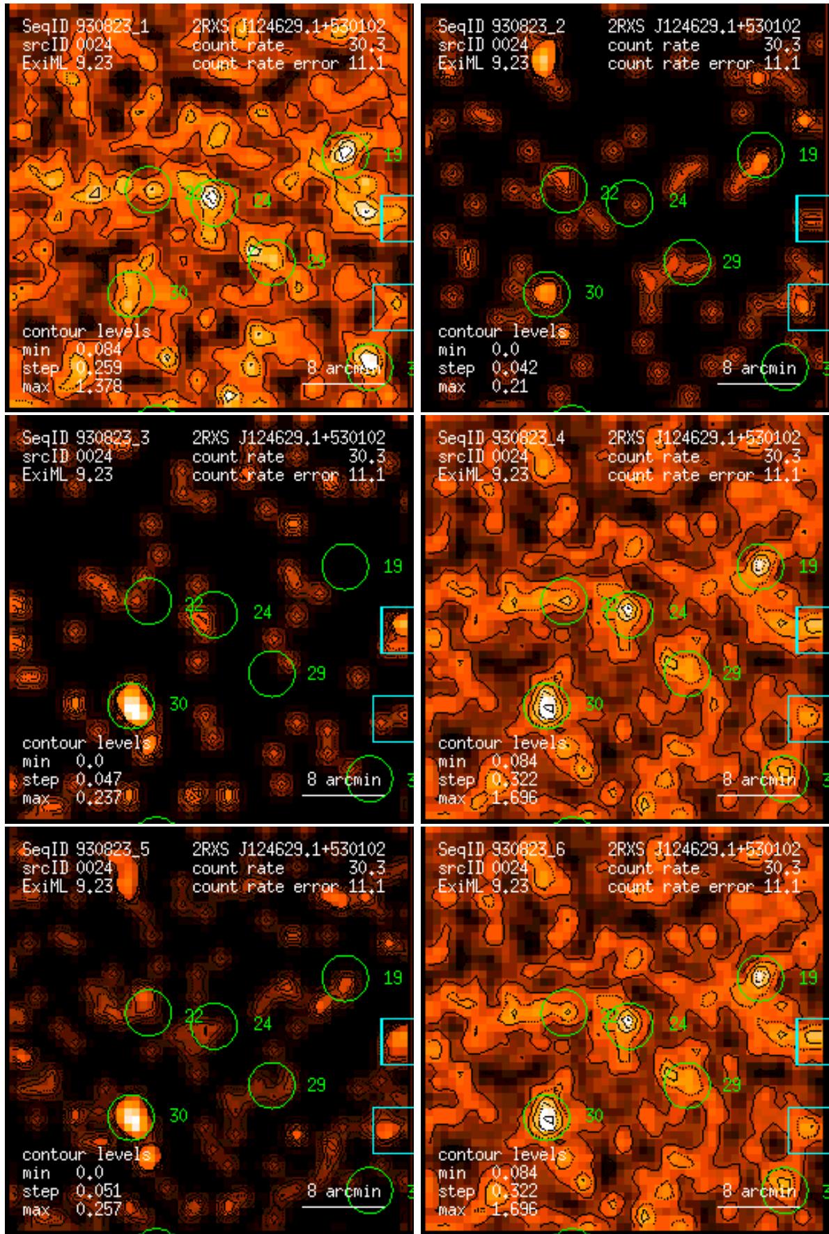
Figure 24: RASS 930823: detection 0024: band rate images, Gaussian filter: (1) PSPC channels 11 – 41, (2) 52 – 90, (3) 91 – 201, (4) 11 – 235, (5) 52 – 201, (6) 11 – 201. Broad band rates in counts/ks. Band rate contour levels in counts/ks/arcmin 2 .
