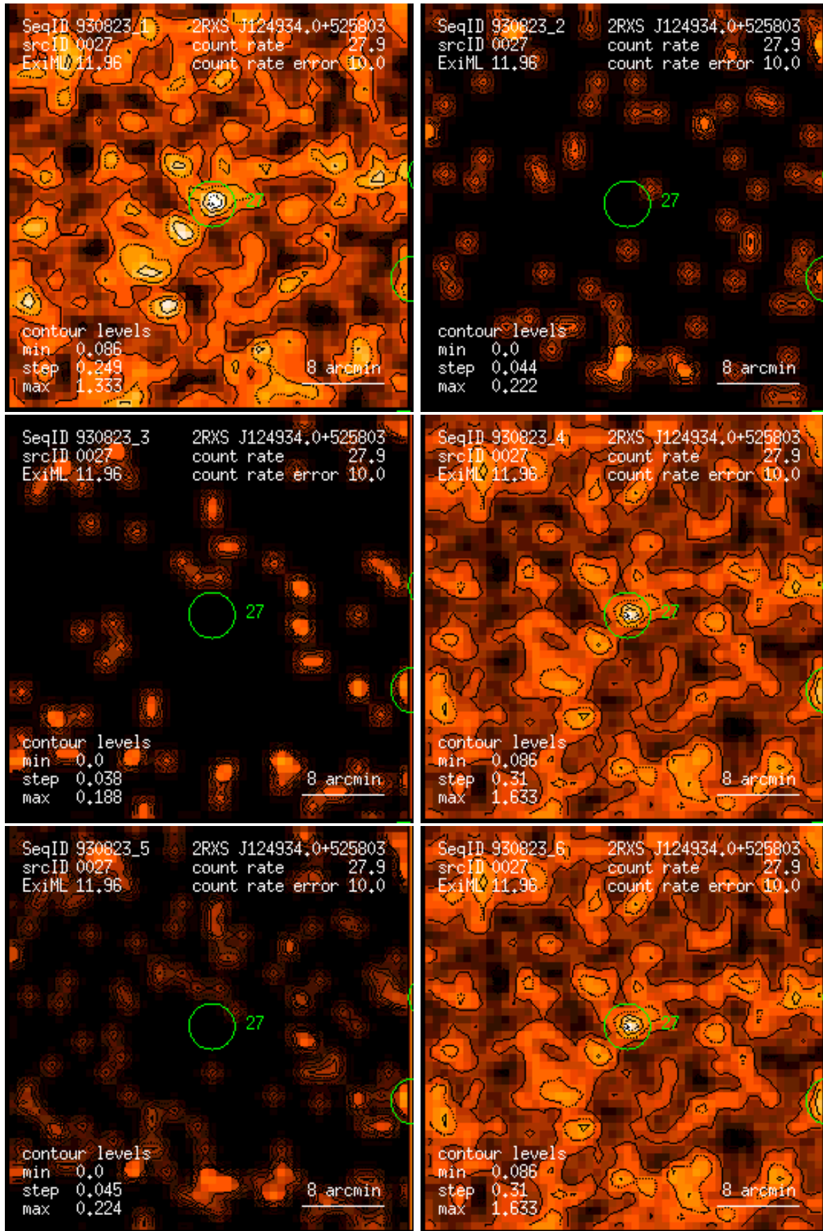
Figure 27: RASS 930823: detection 0027: band rate images, Gaussian filter: (1) PSPC channels 11 – 41, (2) 52 – 90, (3) 91 – 201, (4) 11 – 235, (5) 52 – 201, (6) 11 – 201. Broad band rates in counts/ks. Band rate contour levels in counts/ks/arcmin 2 .
