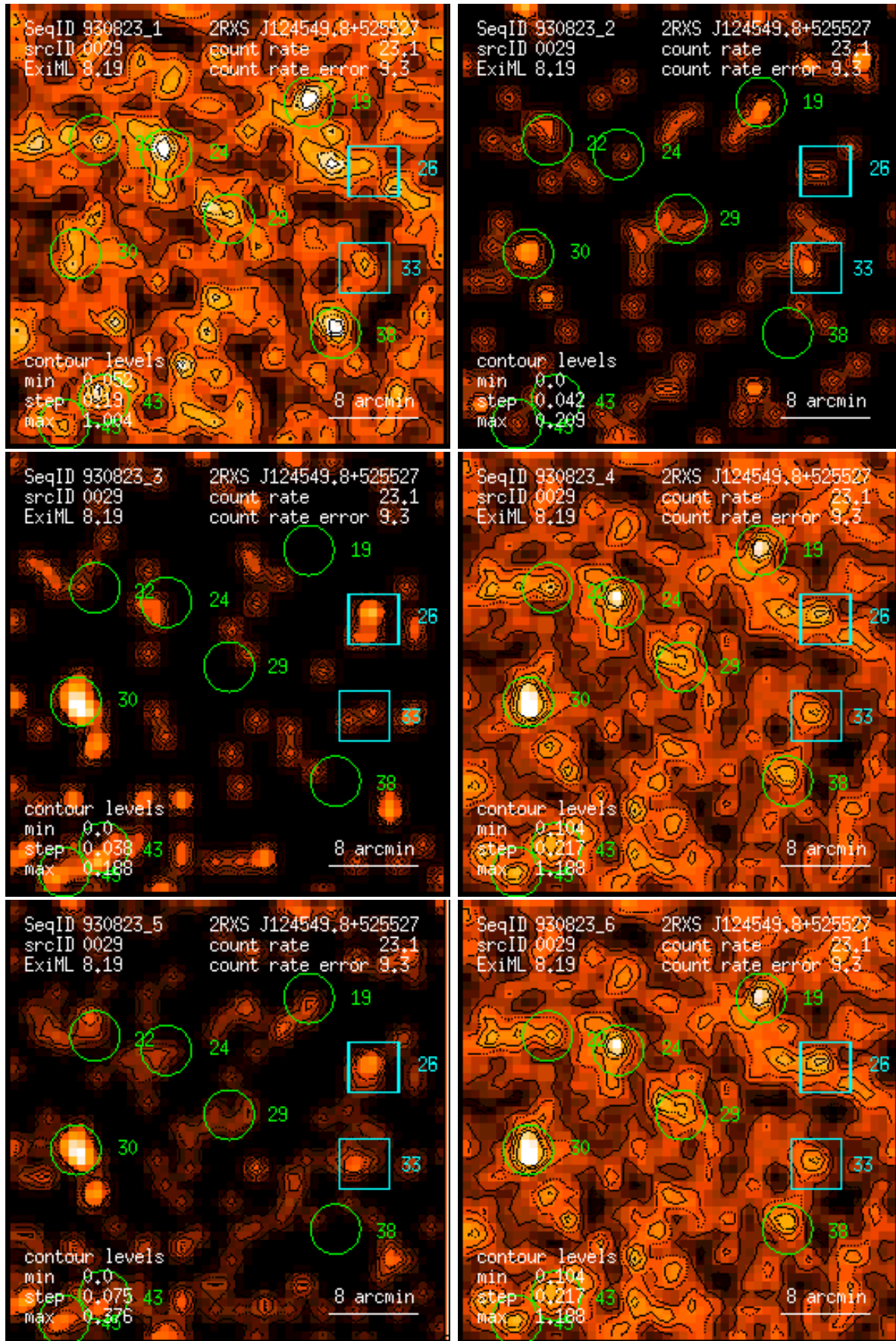
Figure 29: RASS 930823: detection 0029: band rate images, Gaussian filter: (1) PSPC channels 11 – 41, (2) 52 – 90, (3) 91 – 201, (4) 11 – 235, (5) 52 – 201, (6) 11 – 201. Broad band rates in counts/ks. Band rate contour levels in counts/ks/arcmin 2 .
