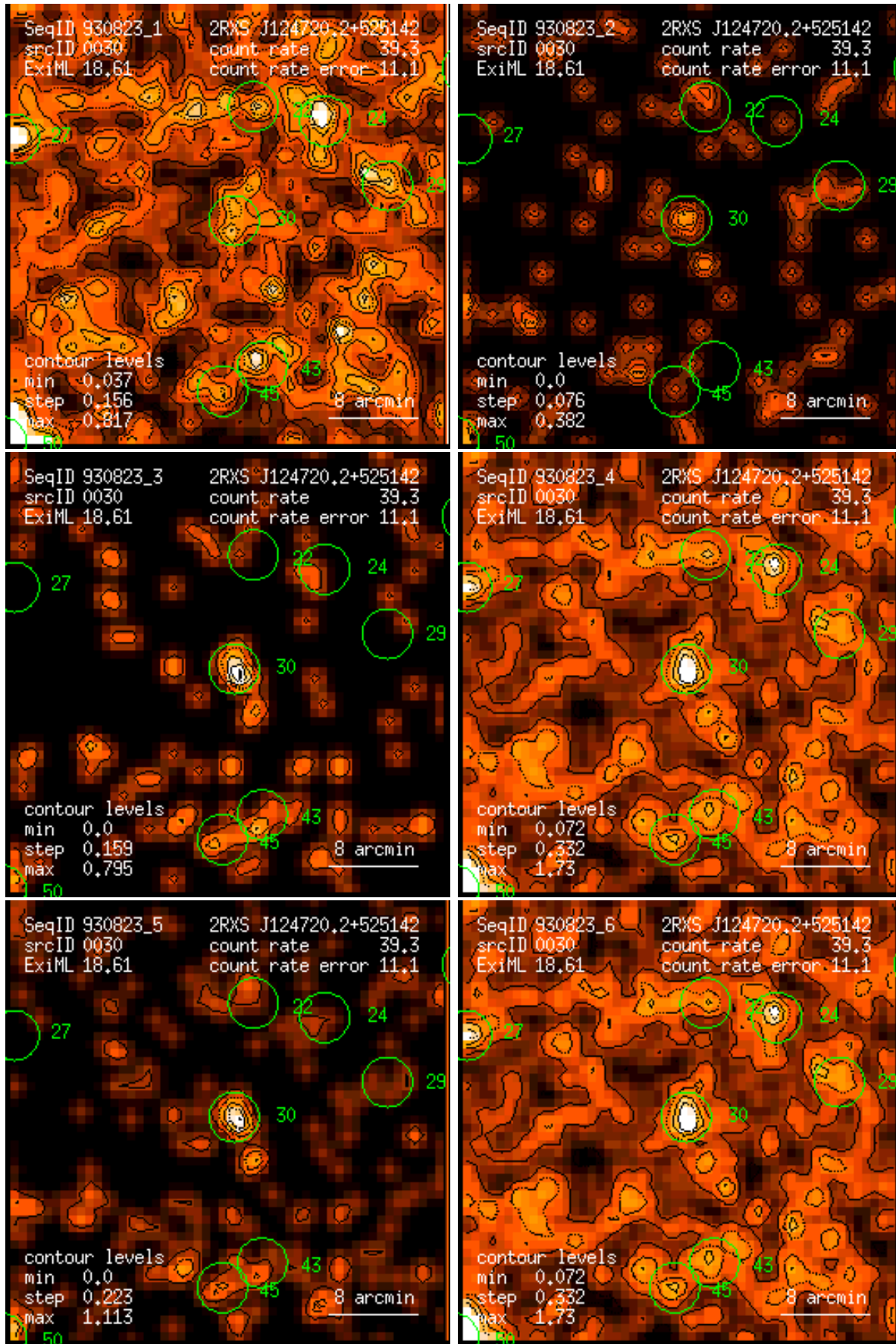
Figure 30: RASS 930823: detection 0030: band rate images, Gaussian filter: (1) PSPC channels 11 – 41, (2) 52 – 90, (3) 91 – 201, (4) 11 – 235, (5) 52 – 201, (6) 11 – 201. Broad band rates in counts/ks. Band rate contour levels in counts/ks/arcmin 2 .
