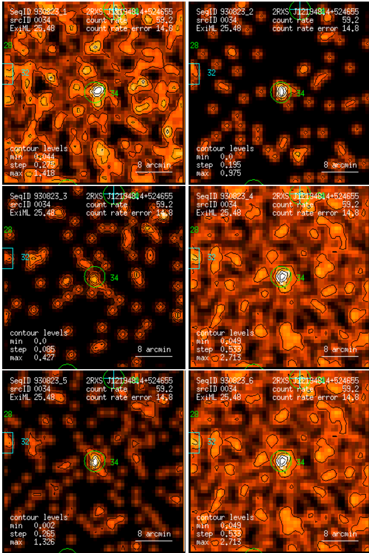
Figure 34: RASS 930823: detection 0034: band rate images, Gaussian filter: (1) PSPC channels 11 – 41, (2) 52 – 90, (3) 91 – 201, (4) 11 – 235, (5) 52 – 201, (6) 11 – 201. Broad band rates in counts/ks. Band rate contour levels in counts/ks/arcmin 2 .
