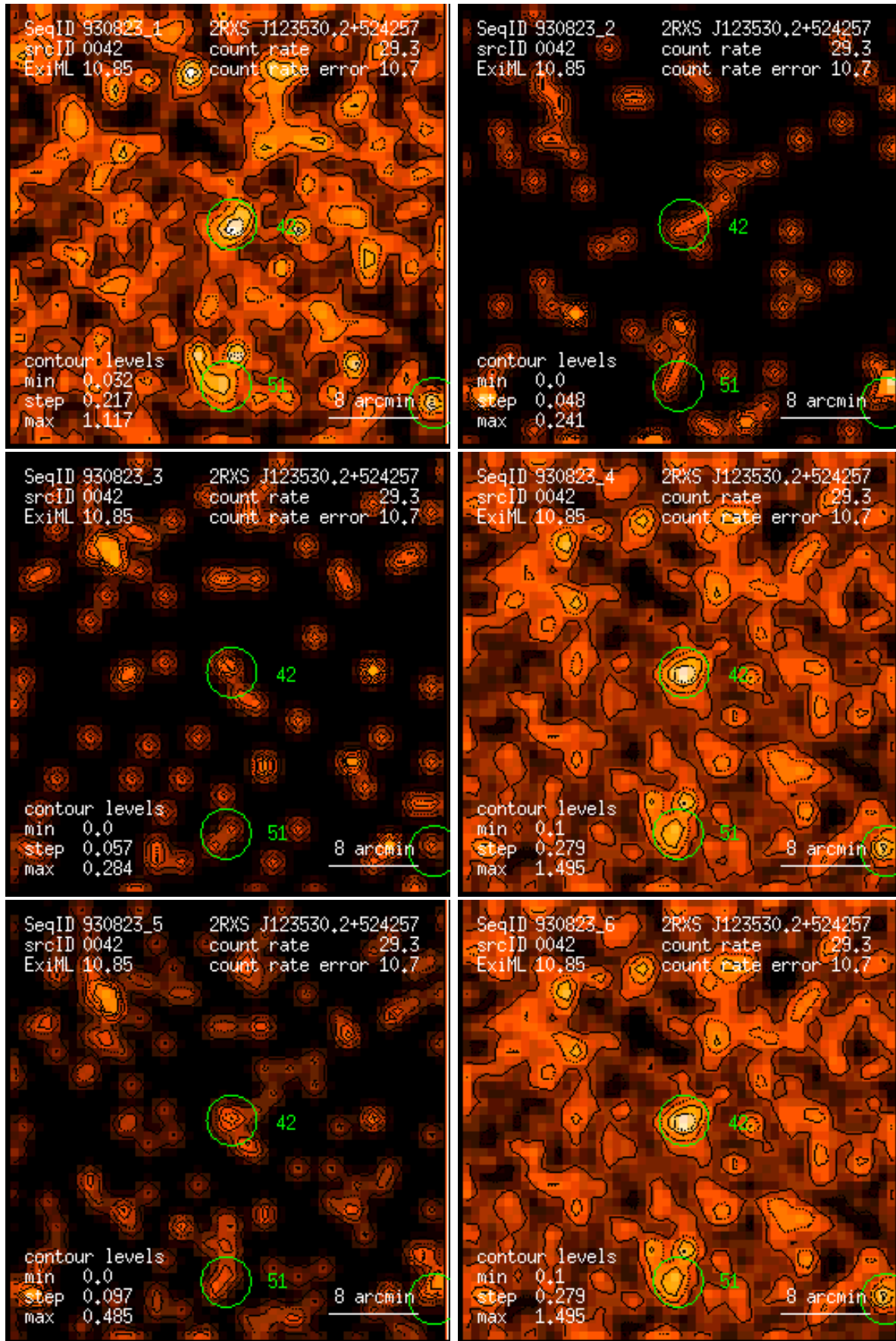
Figure 42: RASS 930823: detection 0042: band rate images, Gaussian filter: (1) PSPC channels 11 – 41, (2) 52 – 90, (3) 91 – 201, (4) 11 – 235, (5) 52 – 201, (6) 11 – 201. Broad band rates in counts/ks. Band rate contour levels in counts/ks/arcmin 2 .
