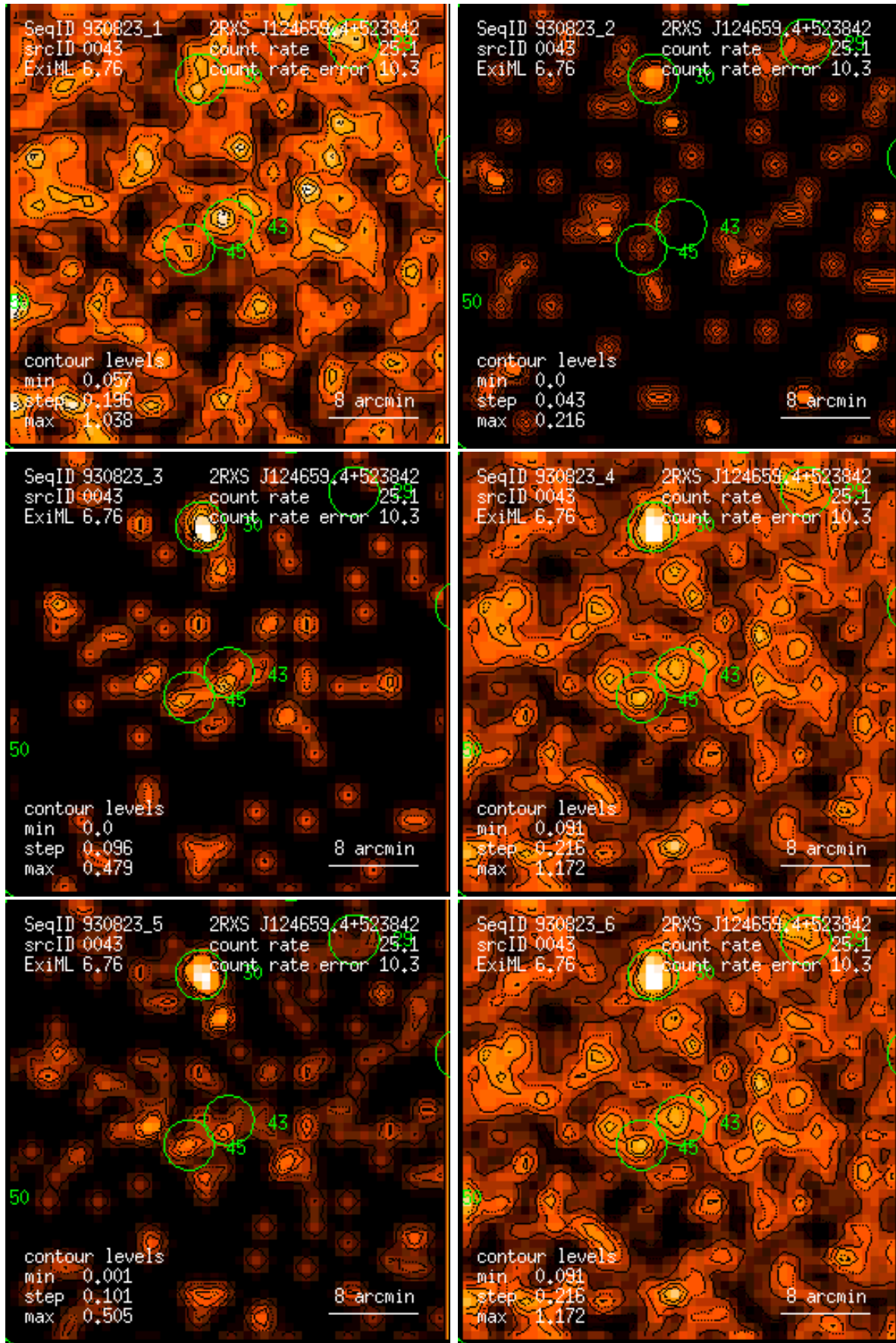
Figure 43: RASS 930823: detection 0043: band rate images, Gaussian filter: (1) PSPC channels 11 – 41, (2) 52 – 90, (3) 91 – 201, (4) 11 – 235, (5) 52 – 201, (6) 11 – 201. Broad band rates in counts/ks. Band rate contour levels in counts/ks/arcmin 2 .
