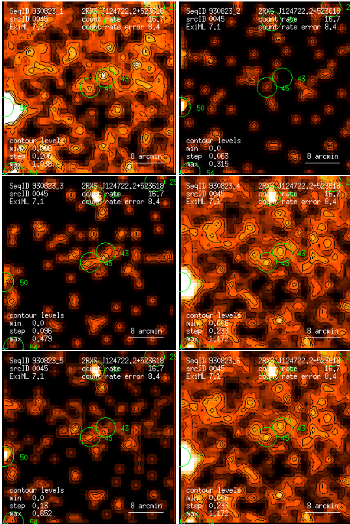
Figure 45: RASS 930823: detection 0045: band rate images, Gaussian filter: (1) PSPC channels 11 – 41, (2) 52 – 90, (3) 91 – 201, (4) 11 – 235, (5) 52 – 201, (6) 11 – 201. Broad band rates in counts/ks. Band rate contour levels in counts/ks/arcmin 2 .
