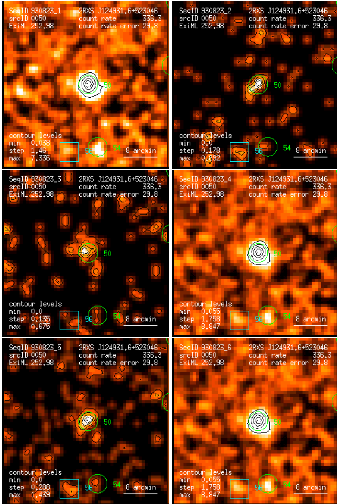
Figure 50: RASS 930823: detection 0050: band rate images, Gaussian filter: (1) PSPC channels 11 – 41, (2) 52 – 90, (3) 91 – 201, (4) 11 – 235, (5) 52 – 201, (6) 11 – 201. Broad band rates in counts/ks. Band rate contour levels in counts/ks/arcmin 2 .
