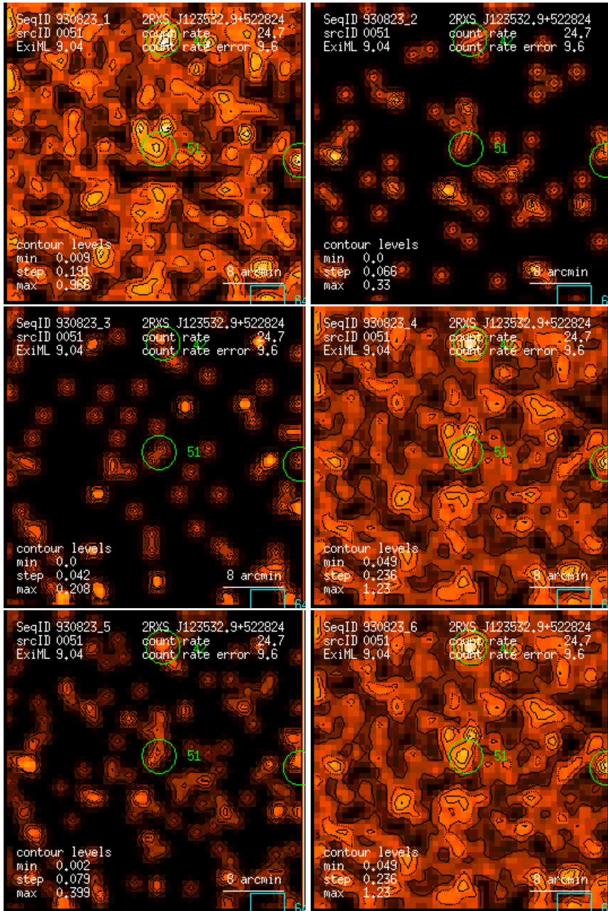
Figure 51: RASS 930823: detection 0051: band rate images, Gaussian filter: (1) PSPC channels 11 – 41, (2) 52 – 90, (3) 91 – 201, (4) 11 – 235, (5) 52 – 201, (6) 11 – 201. Broad band rates in counts/ks. Band rate contour levels in counts/ks/arcmin 2 .
