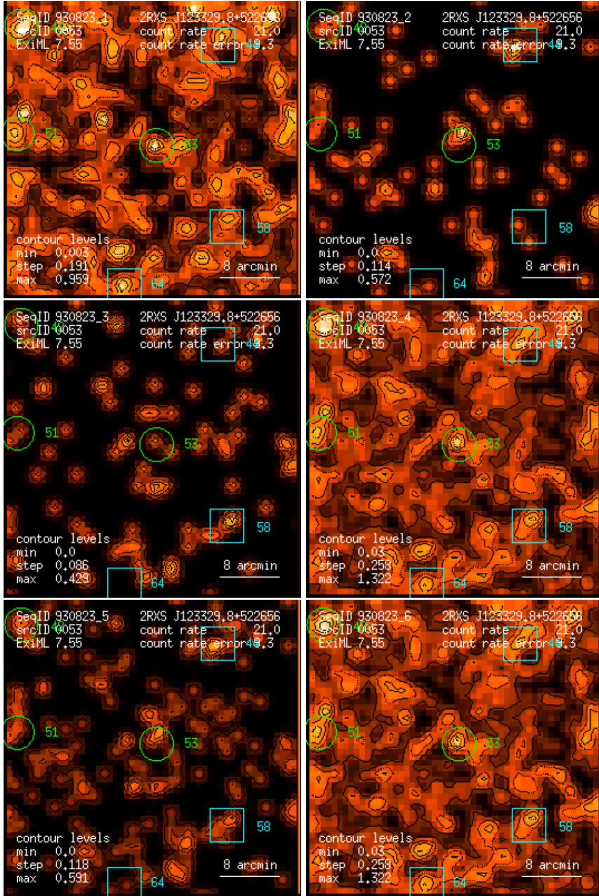
Figure 53: RASS 930823: detection 0053: band rate images, Gaussian filter: (1) PSPC channels 11 – 41, (2) 52 – 90, (3) 91 – 201, (4) 11 – 235, (5) 52 – 201, (6) 11 – 201. Broad band rates in counts/ks. Band rate contour levels in counts/ks/arcmin 2 .
