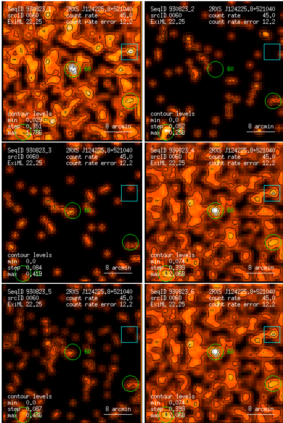
Figure 60: RASS 930823: detection 0060: band rate images, Gaussian filter: (1) PSPC channels 11 – 41, (2) 52 – 90, (3) 91 – 201, (4) 11 – 235, (5) 52 – 201, (6) 11 – 201. Broad band rates in counts/ks. Band rate contour levels in counts/ks/arcmin 2 .
