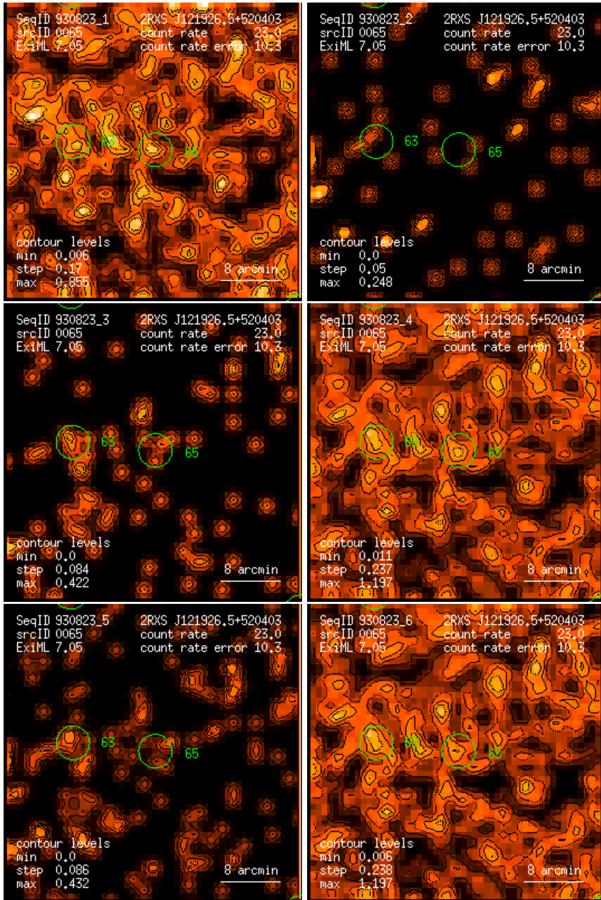
Figure 65: RASS 930823: detection 0065: band rate images, Gaussian filter: (1) PSPC channels 11 – 41, (2) 52 – 90, (3) 91 – 201, (4) 11 – 235, (5) 52 – 201, (6) 11 – 201. Broad band rates in counts/ks. Band rate contour levels in counts/ks/arcmin 2 .
