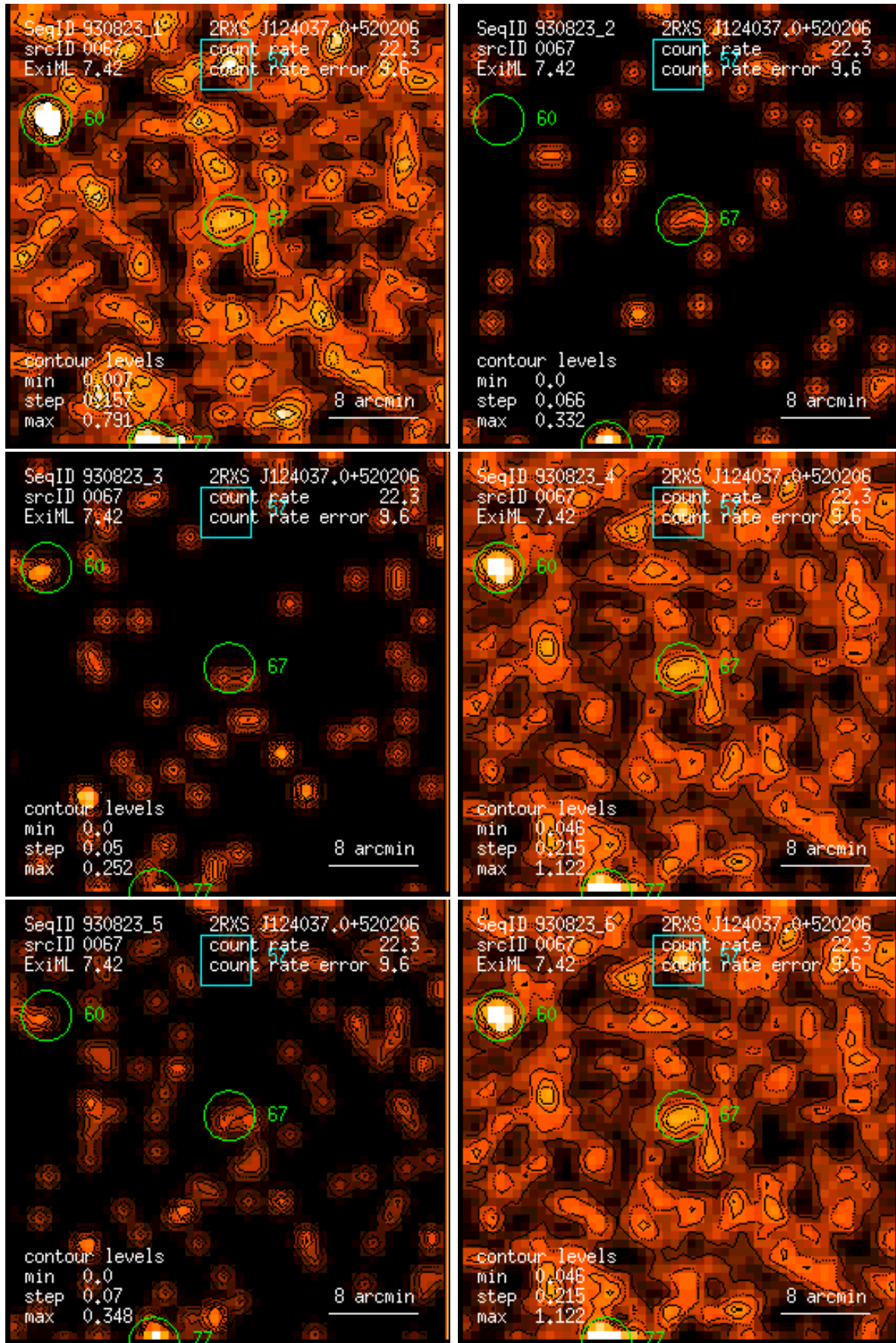
Figure 67: RASS 930823: detection 0067: band rate images, Gaussian filter: (1) PSPC channels 11 – 41, (2) 52 – 90, (3) 91 – 201, (4) 11 – 235, (5) 52 – 201, (6) 11 – 201. Broad band rates in counts/ks. Band rate contour levels in counts/ks/arcmin 2 .
