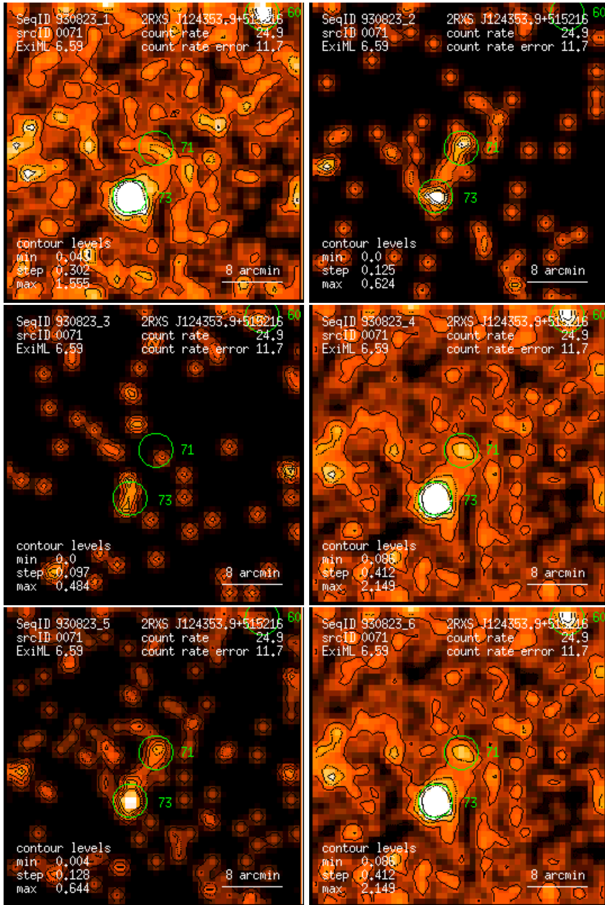
Figure 71: RASS 930823: detection 0071: band rate images, Gaussian filter: (1) PSPC channels 11 – 41, (2) 52 – 90, (3) 91 – 201, (4) 11 – 235, (5) 52 – 201, (6) 11 – 201. Broad band rates in counts/ks. Band rate contour levels in counts/ks/arcmin 2 .
