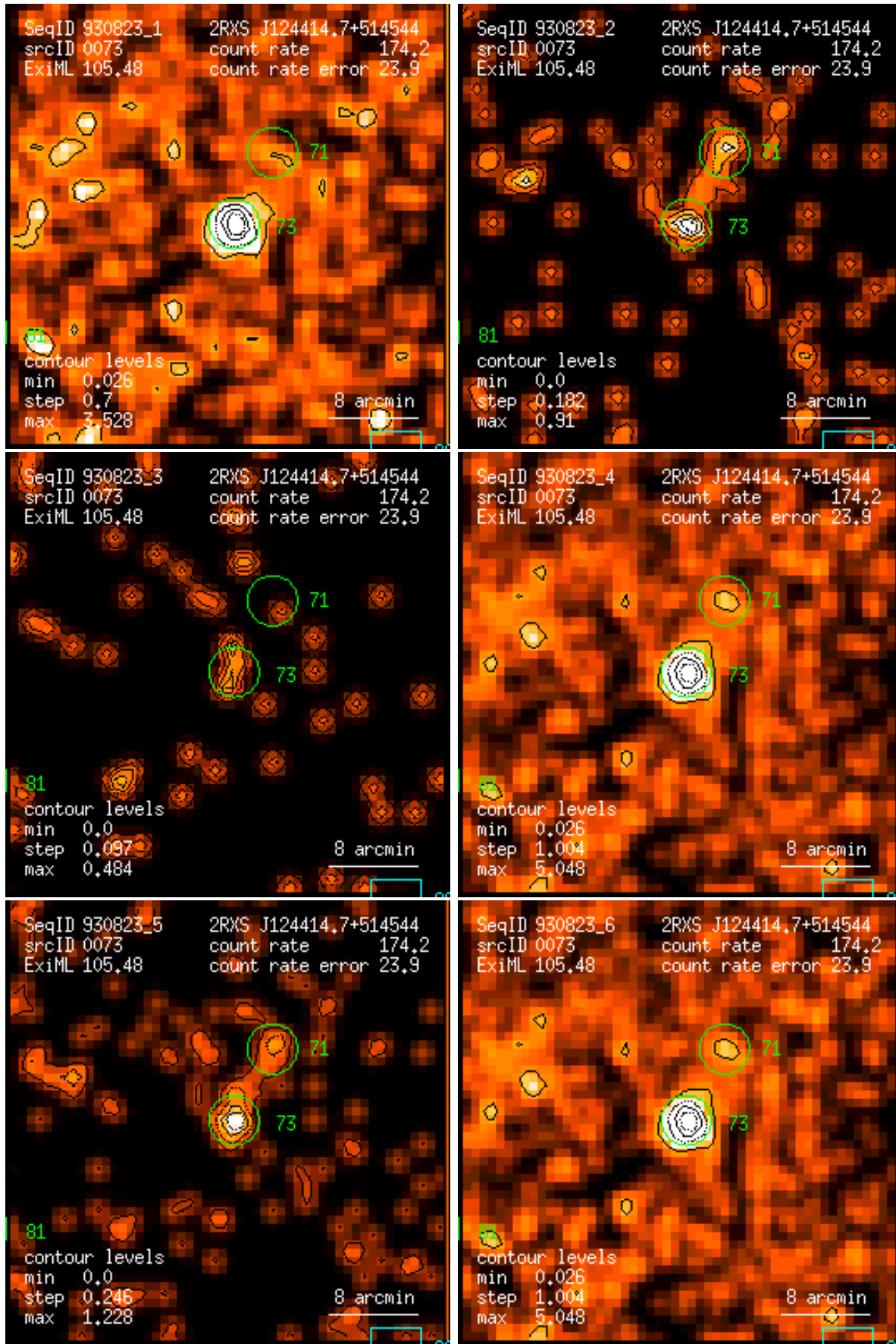
Figure 73: RASS 930823: detection 0073: band rate images, Gaussian filter: (1) PSPC channels 11 – 41, (2) 52 – 90, (3) 91 – 201, (4) 11 – 235, (5) 52 – 201, (6) 11 – 201. Broad band rates in counts/ks. Band rate contour levels in counts/ks/arcmin 2 .
