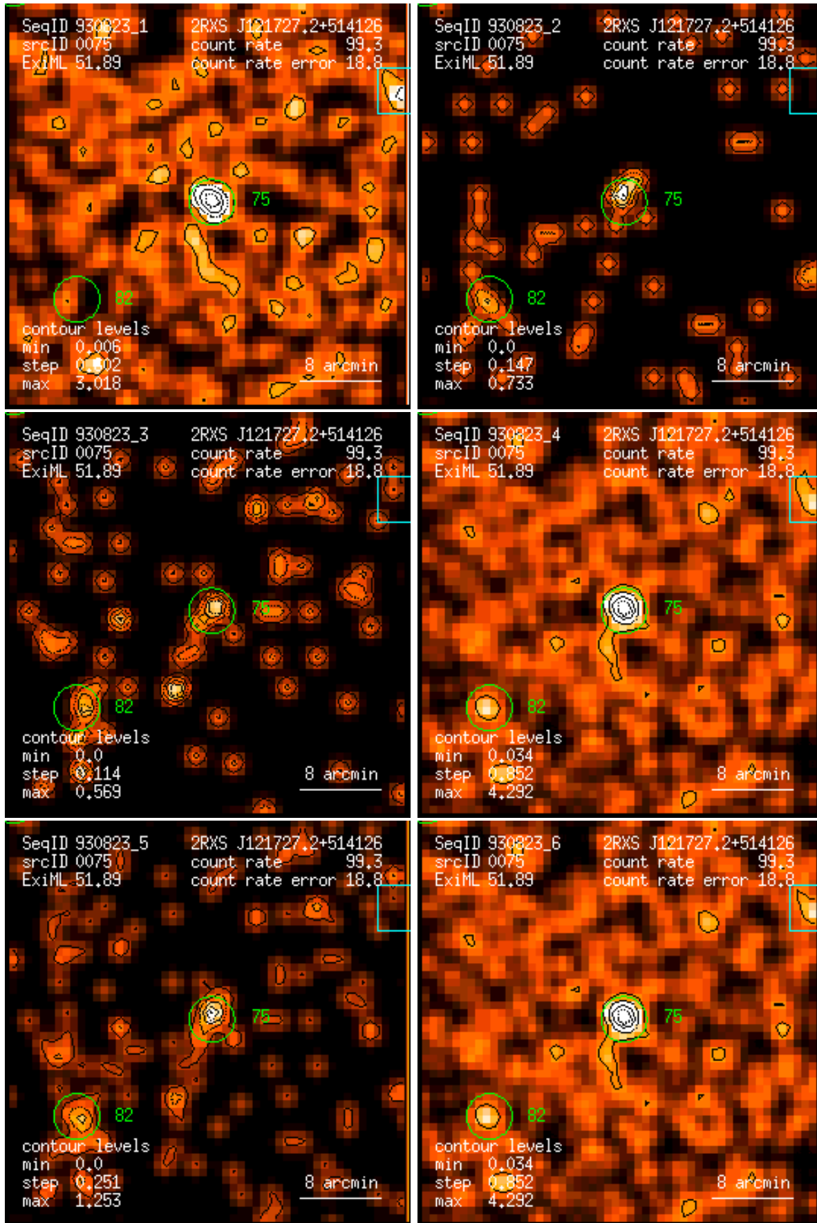
Figure 75: RASS 930823: detection 0075: band rate images, Gaussian filter: (1) PSPC channels 11 – 41, (2) 52 – 90, (3) 91 – 201, (4) 11 – 235, (5) 52 – 201, (6) 11 – 201. Broad band rates in counts/ks. Band rate contour levels in counts/ks/arcmin 2 .
